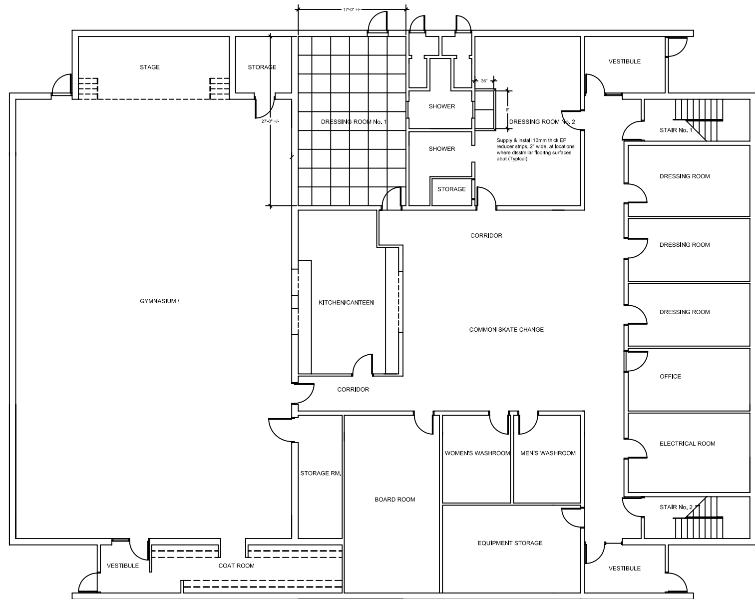
BUILDING FLOOR PLAN SCALE: NOT TO SCALE
