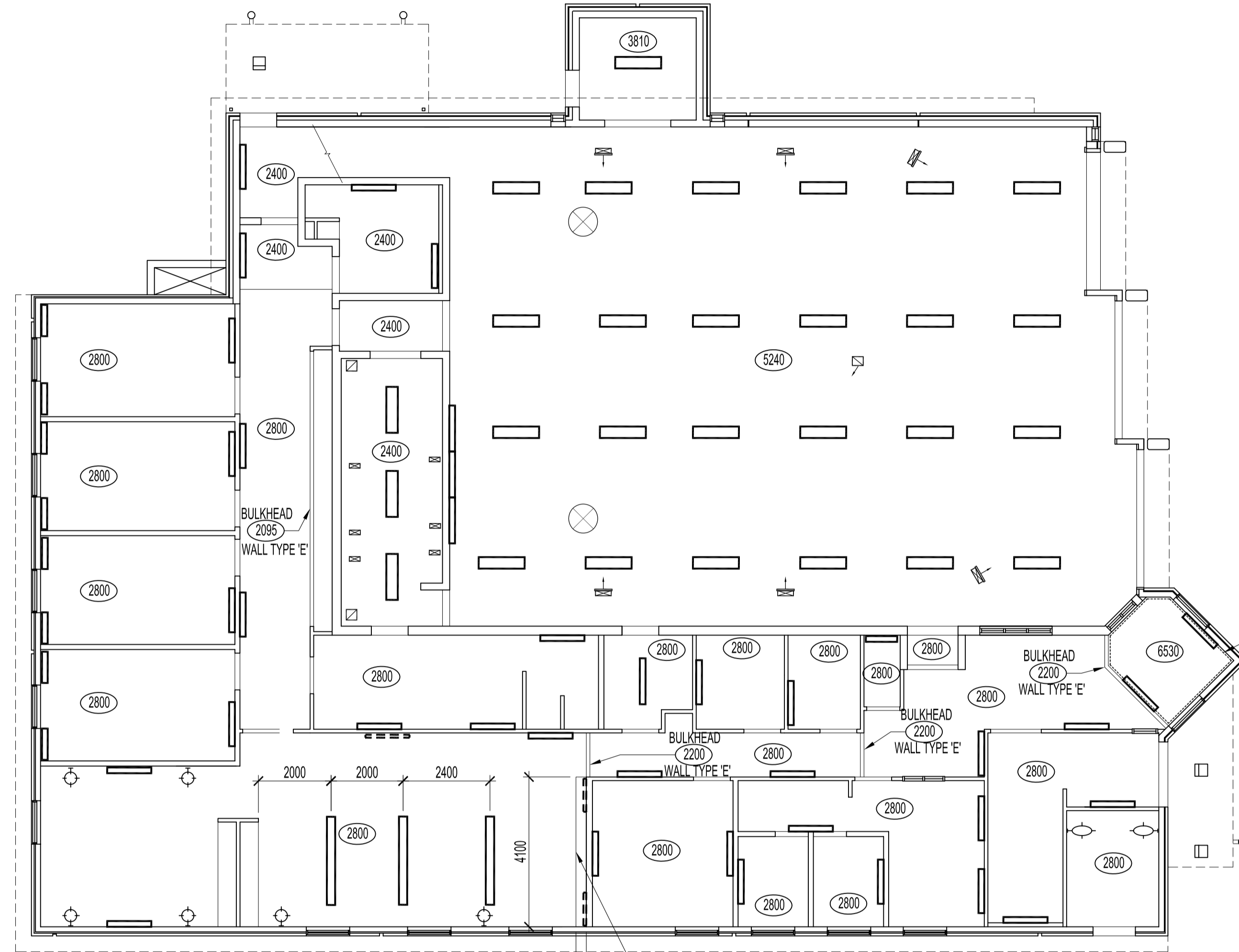
2 MAIN FLOOR PLAN - REFLECTED CEILING A5 SCALE 1:100
