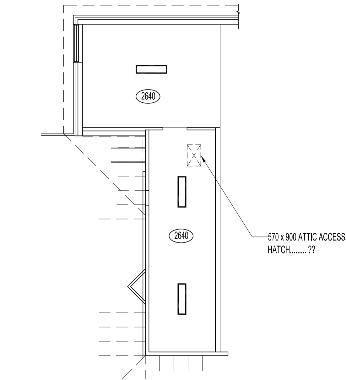
1 MEZZANINE FLOOR PLAN - REFLECTED CEILING A5 SCALE 1:100
