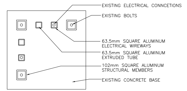
PLAN VIEW AT BASE
