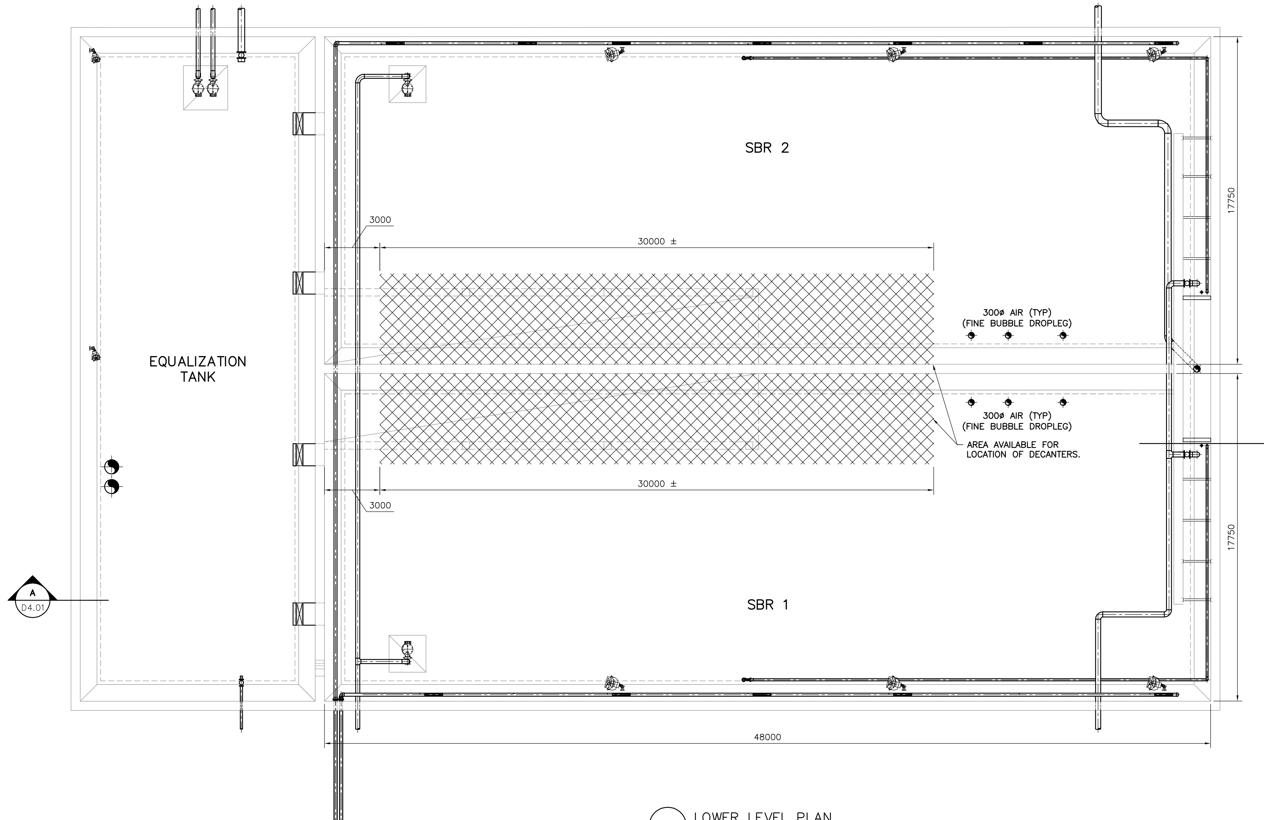
LOWER LEVEL PLAN SCALE 1:125
