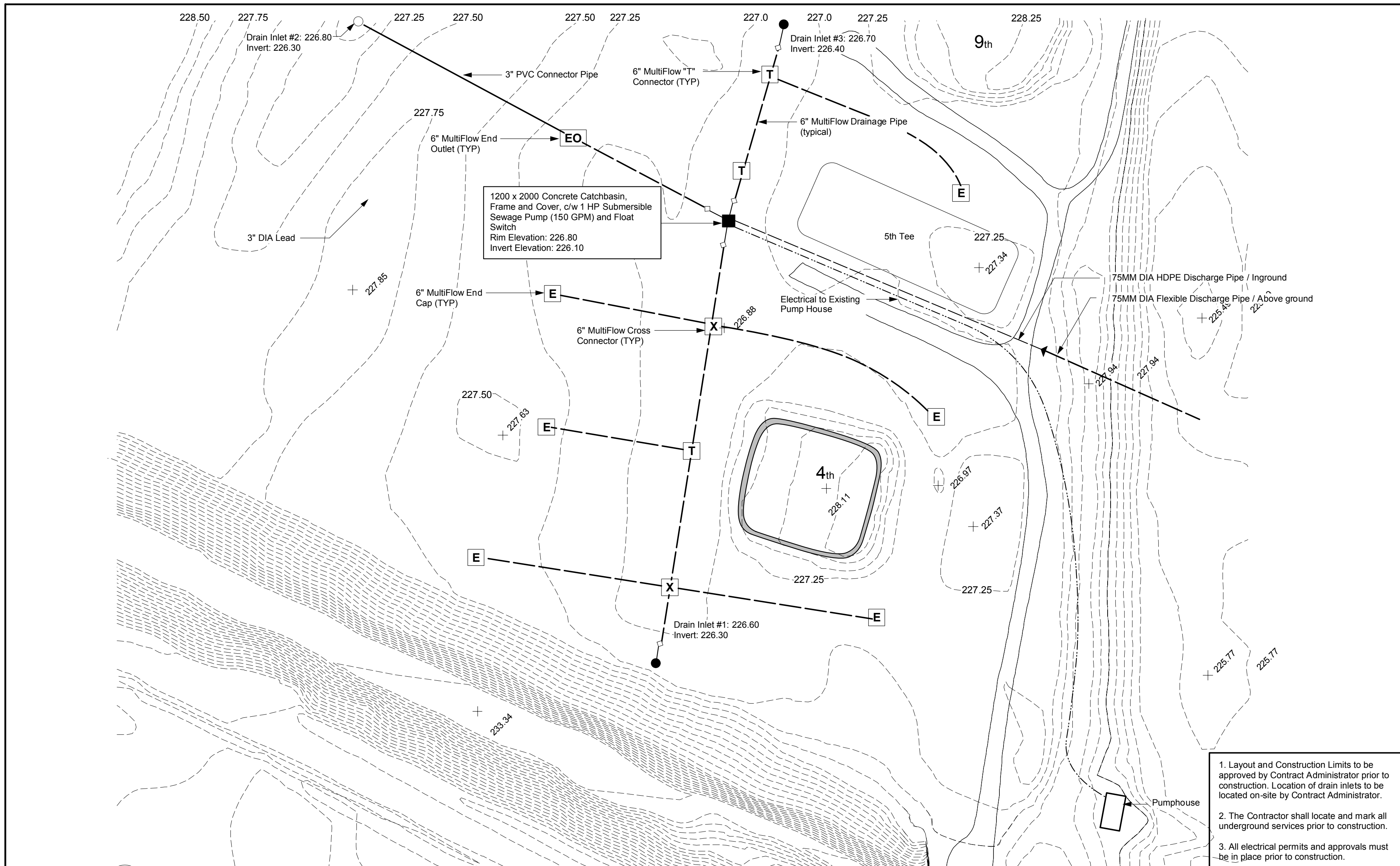
1 Proposed Drainage Works 1:500
