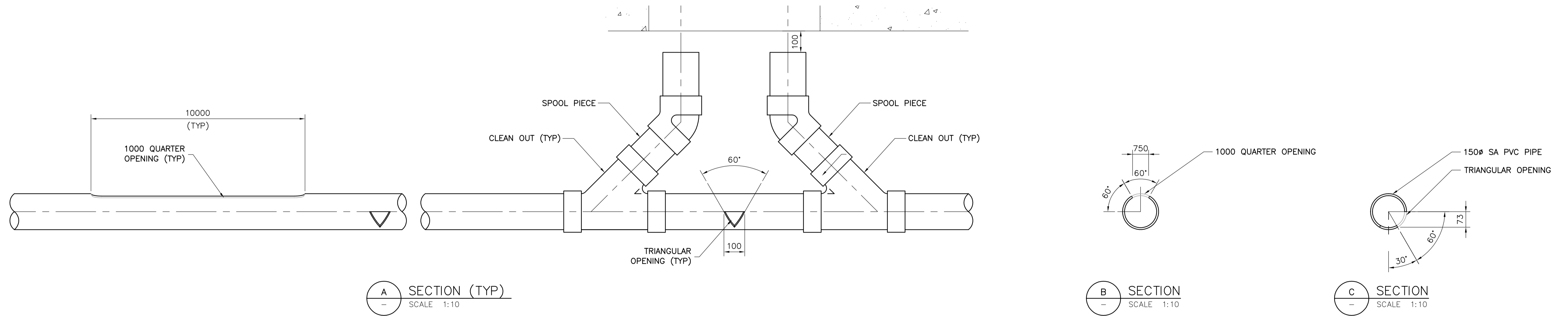
1 DETAIL P13.01 SCALE 1:25
