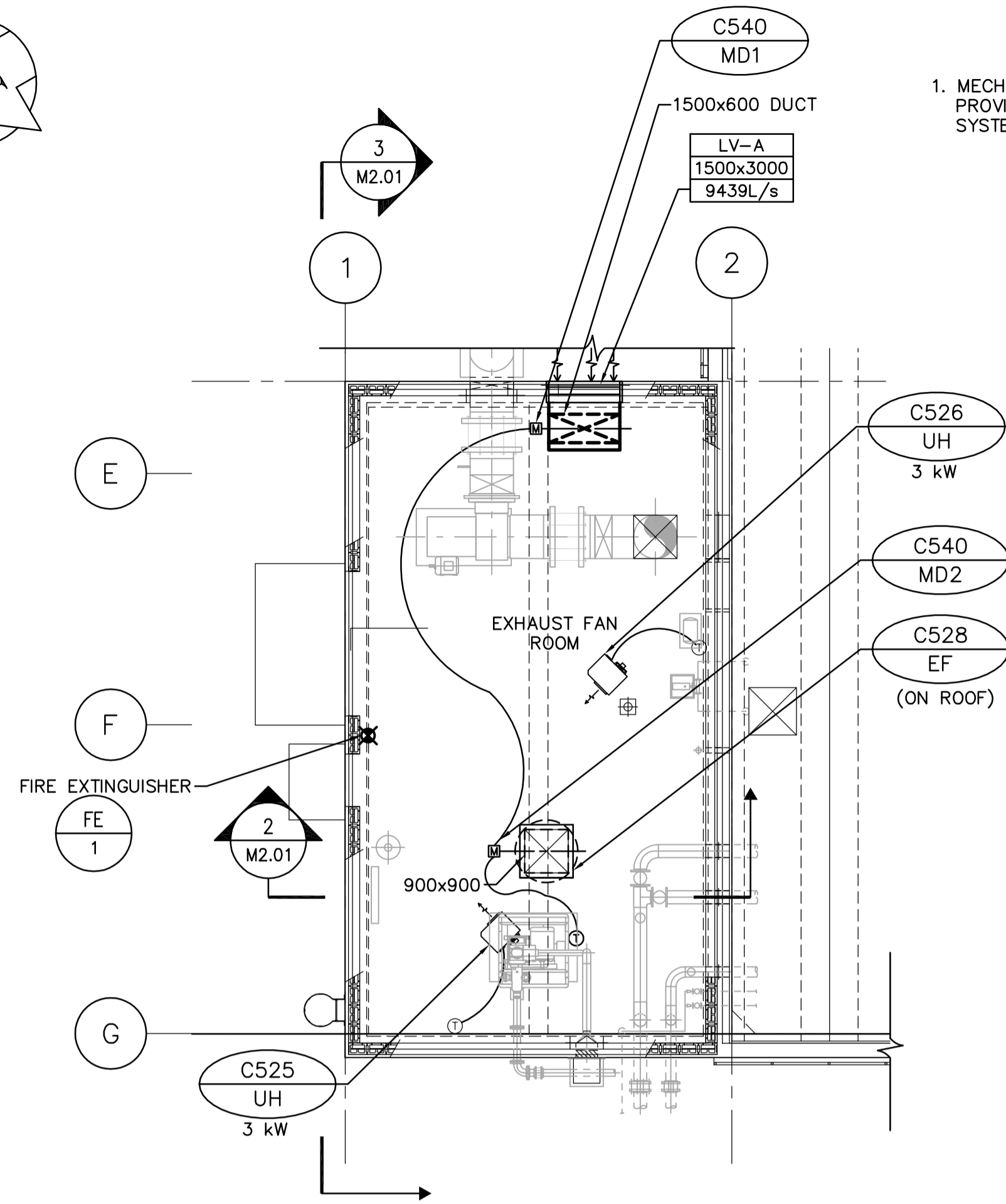
1 EXHAUST FAN BUILDING - HVAC PLAN M1.02 SCALE 1:100
