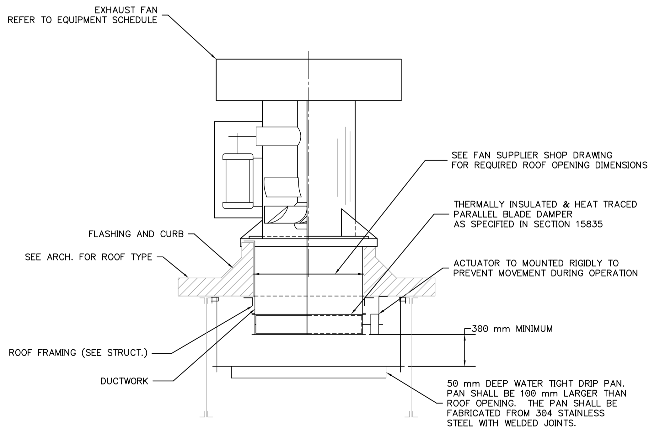
4 EXHAUST FAN ON ROOF DETAIL M1.02 SCALE N.T.S.
