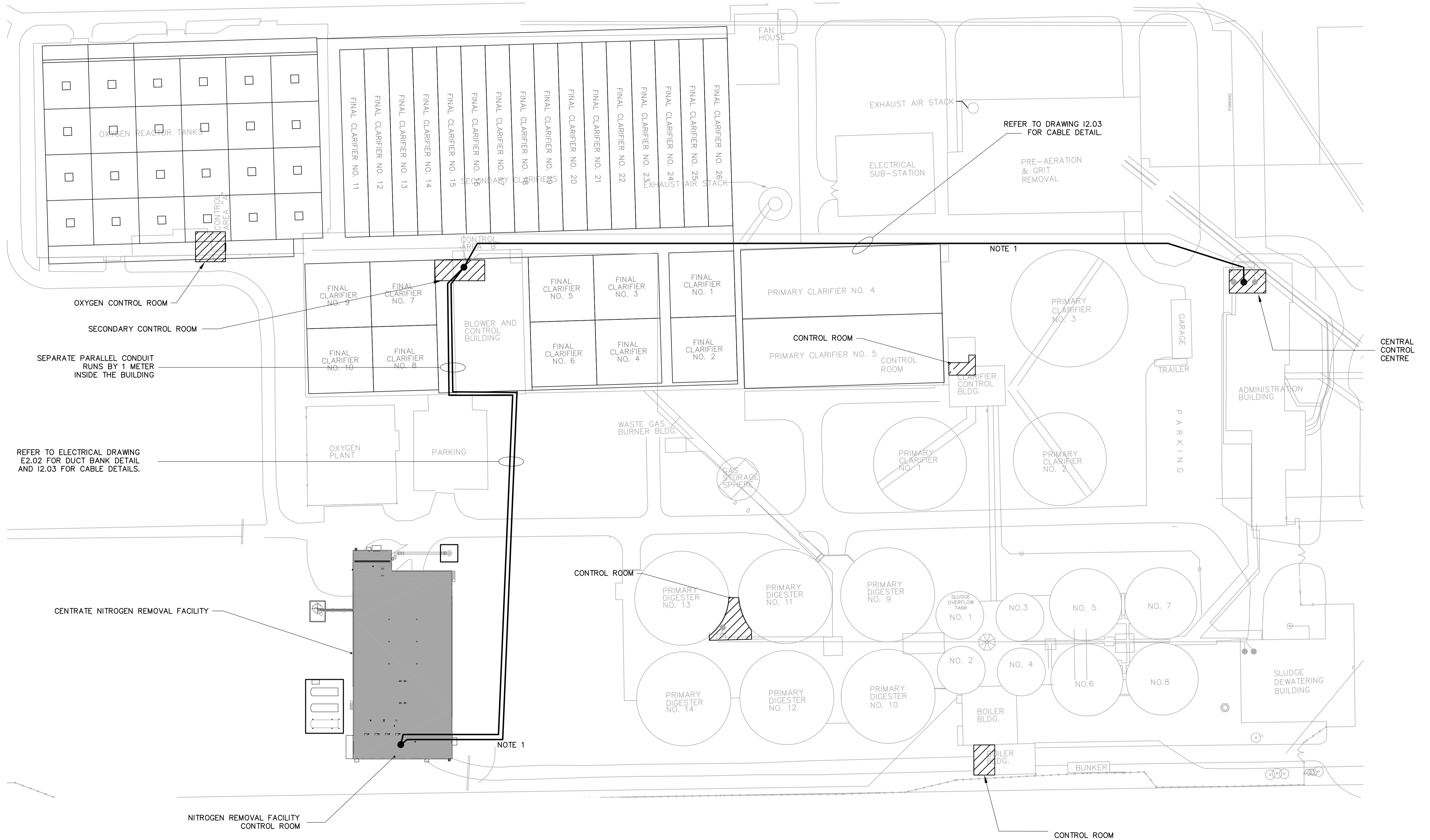
PCU WORKSTATION SITE PLAN SCALE 1:750
