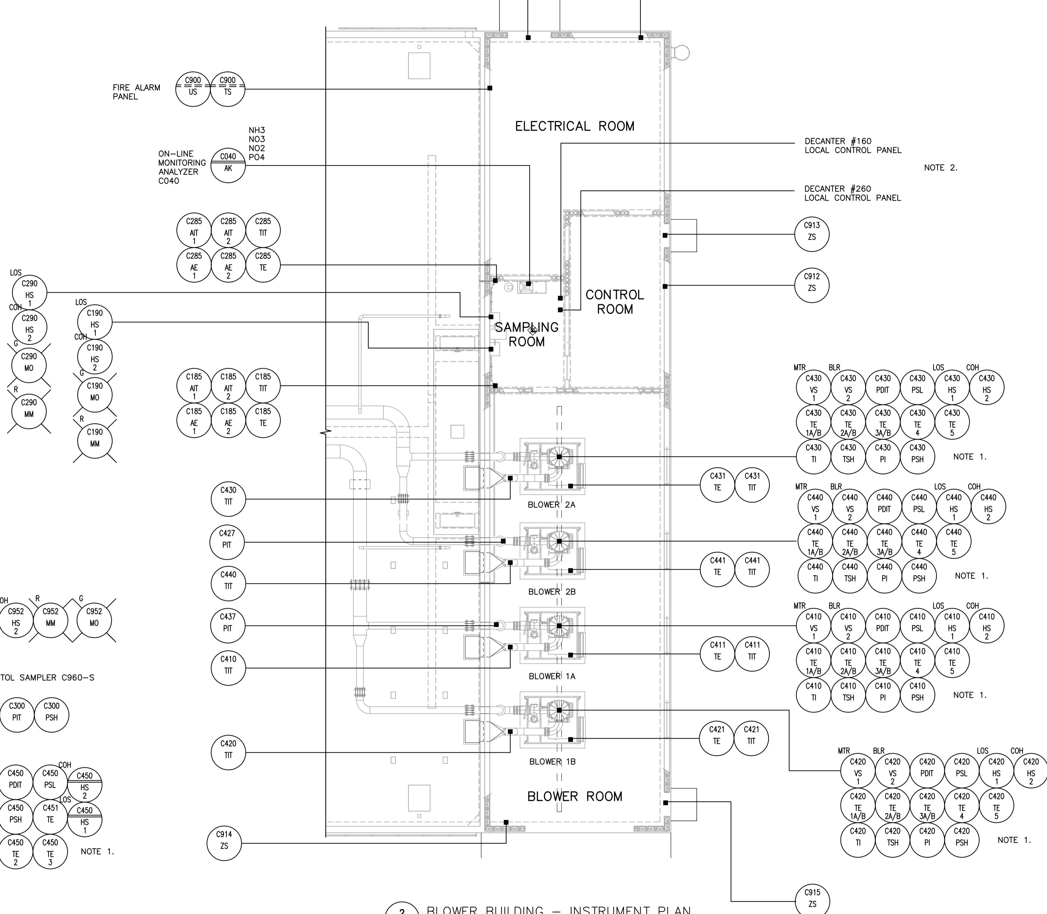
2 BLOWER BUILDING – INSTRUMENT PLAN SCALE 1:100
