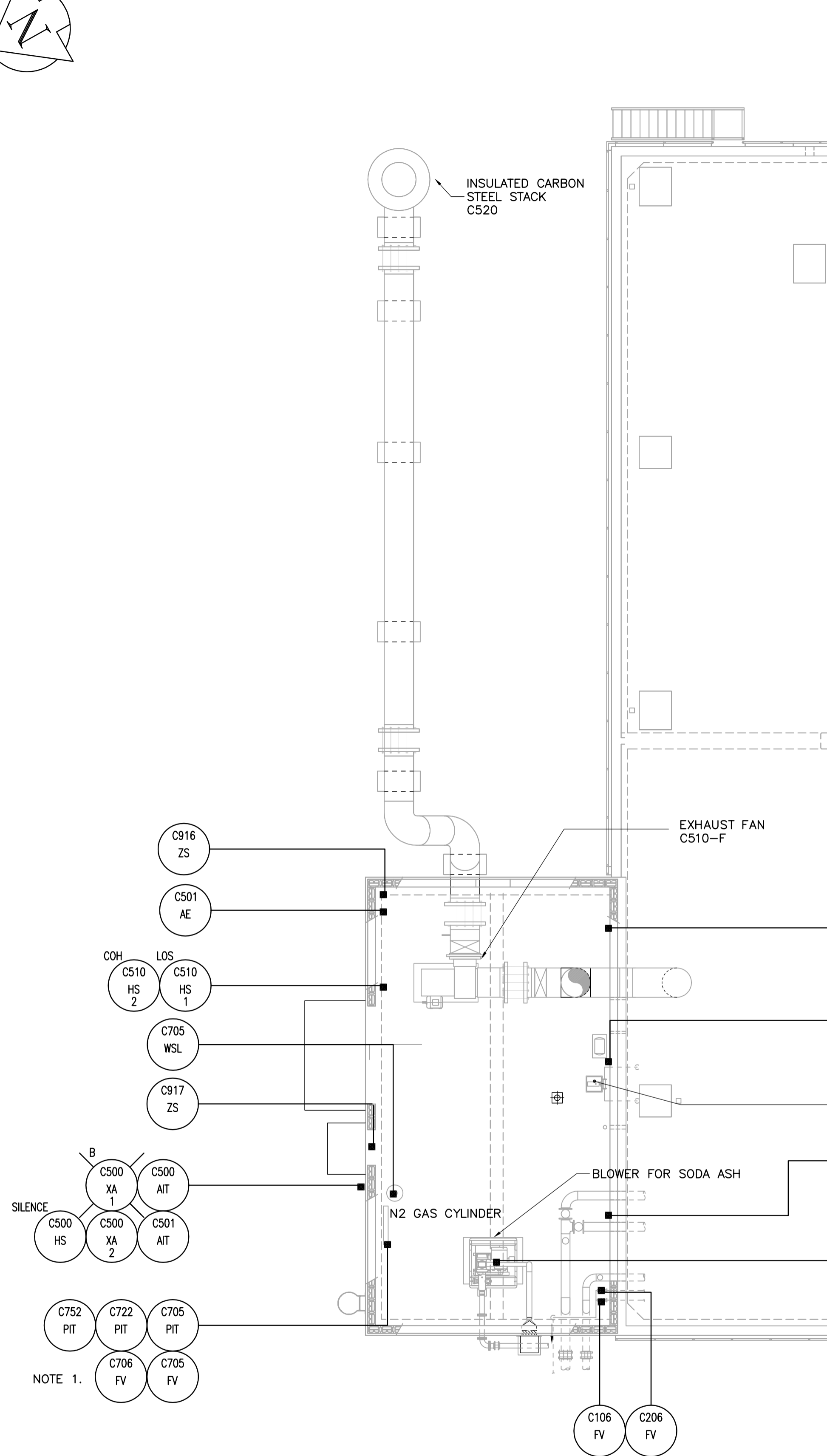
1 EXHAUST FAN ROOM – INSTRUMENT PLAN SCALE 1:100
