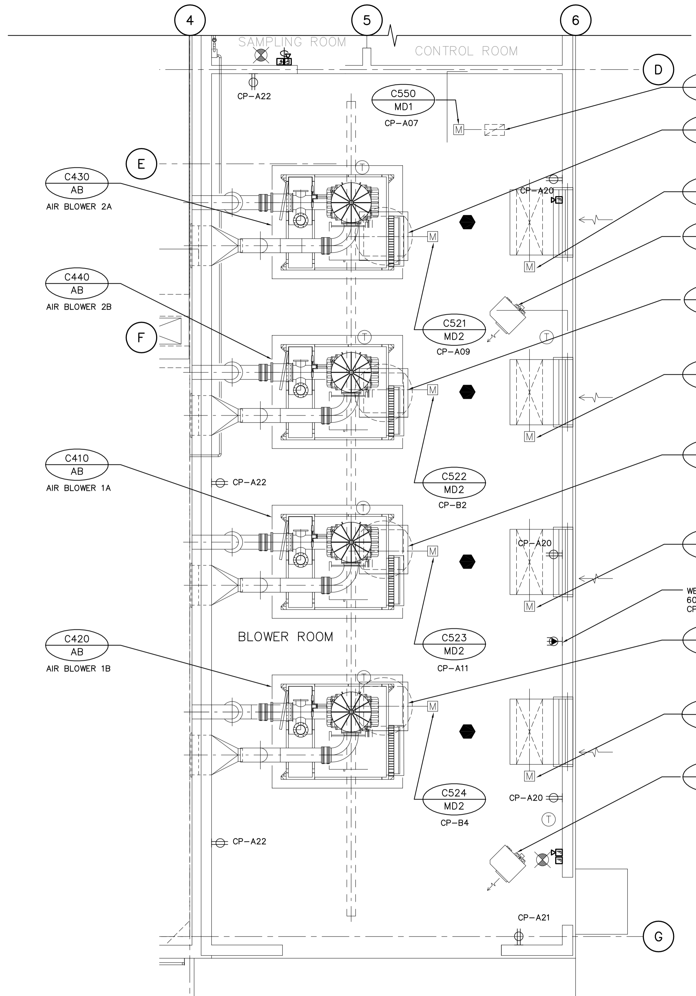
BLOWER ROOM - POWER CONTROL PLAN SCALE: 1:50
