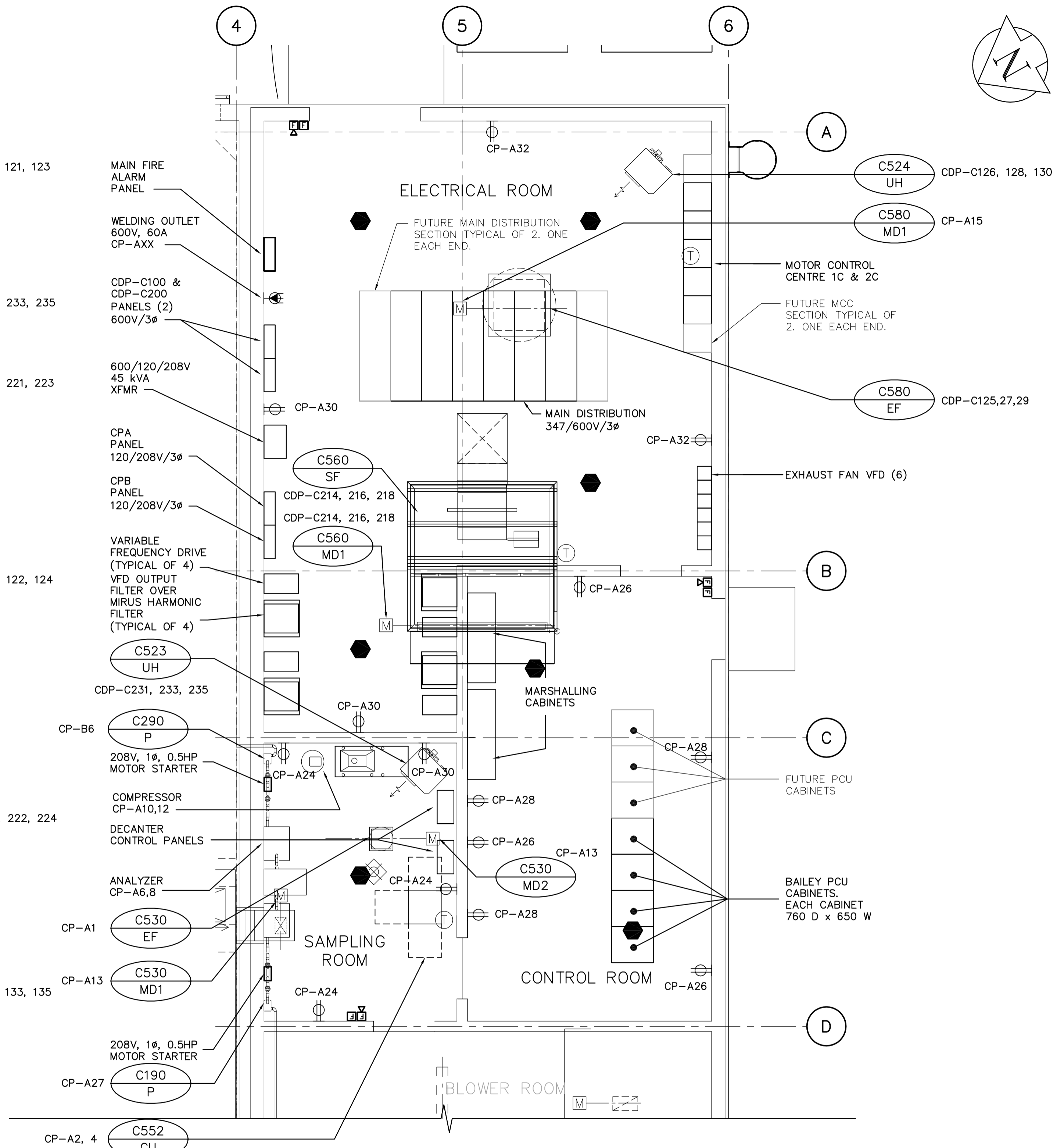
ELECTRICAL ROOM - POWER CONTROL PLAN SCALE: 1:50
