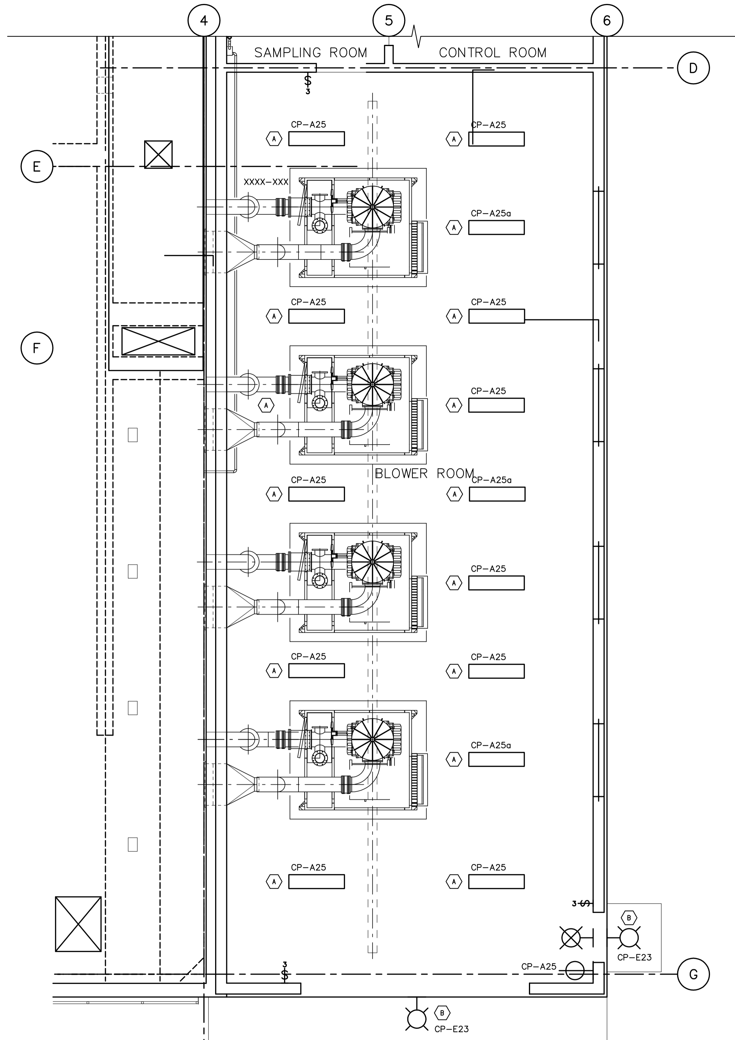
BLOWER ROOM - LIGHTING & SYSTEM PLAN SCALE: 1:50
