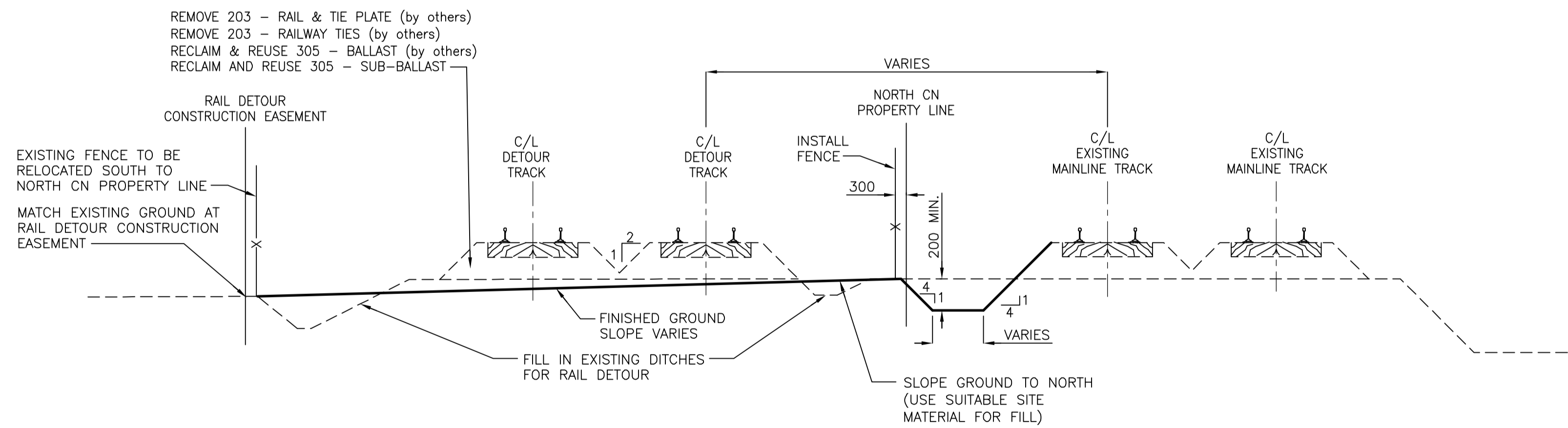
CN RAIL MAINLINE DETOUR TYPICAL TRACK SECTION - FINISHED GRADING N.T.S.
