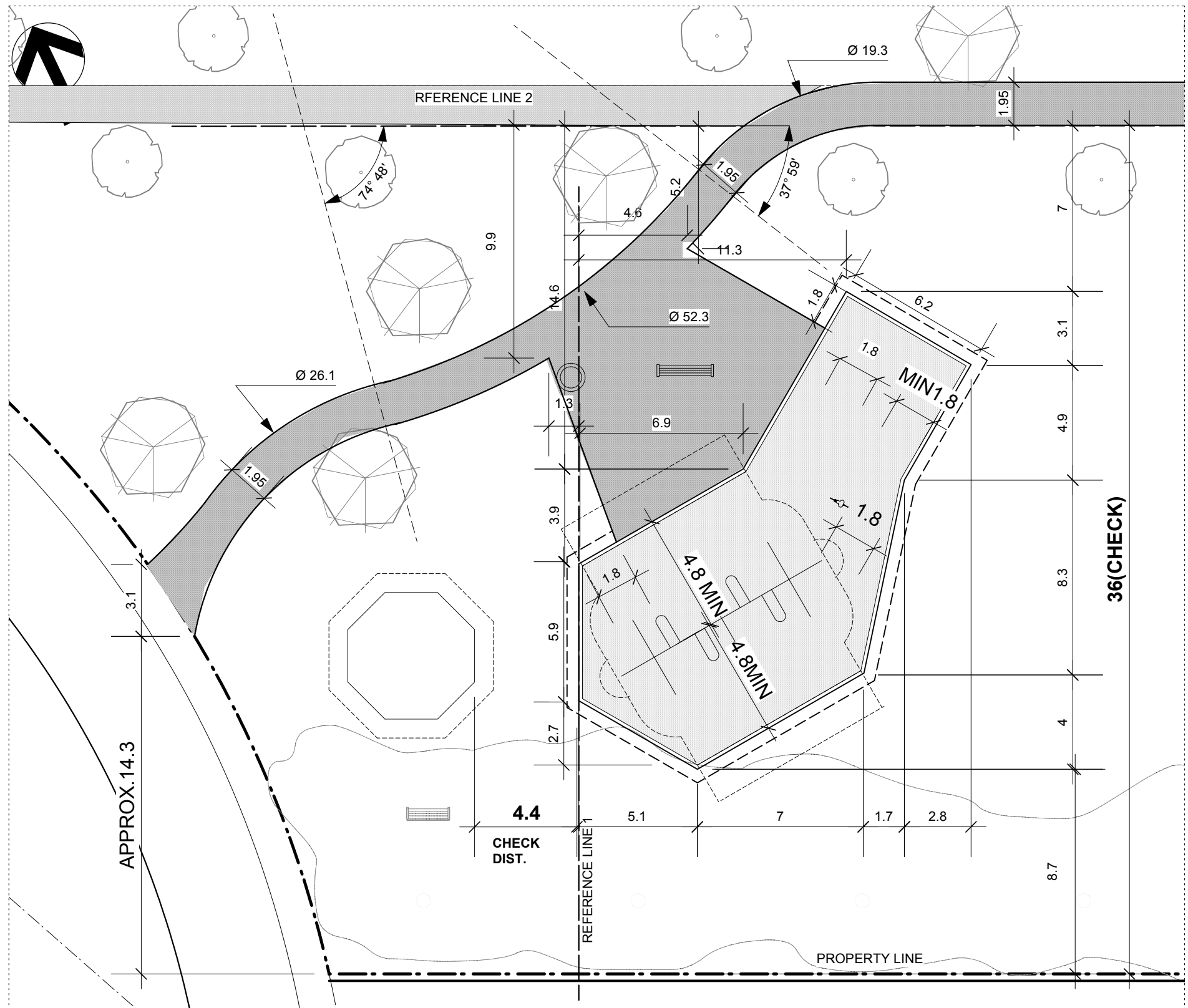
LAYOUT FOR NEW PLAY AREA
