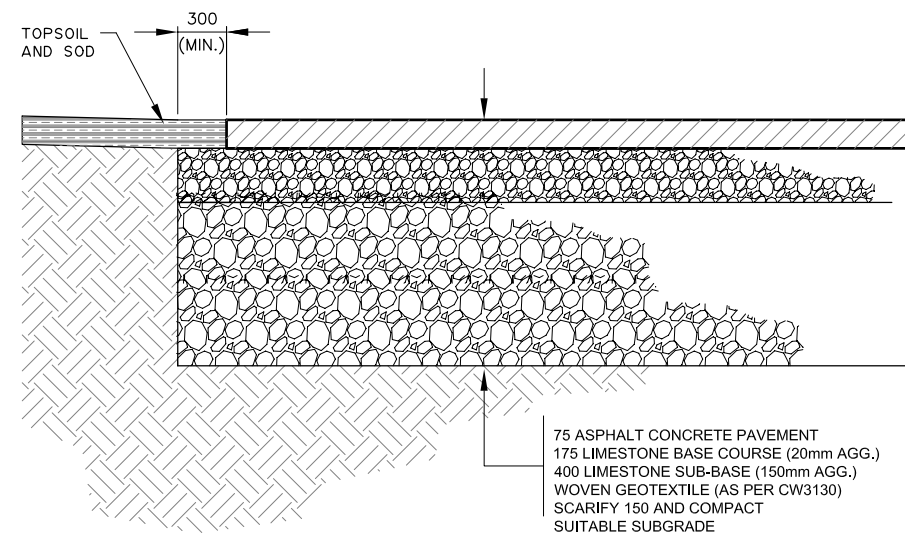
HEAVY DUTY PAVEMENT STRUCTURE N.T.S.
