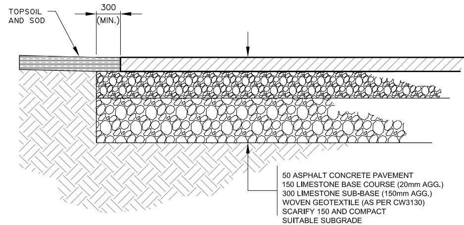
LIGHT DUTY PAVEMENT STRUCTURE N.T.S.
