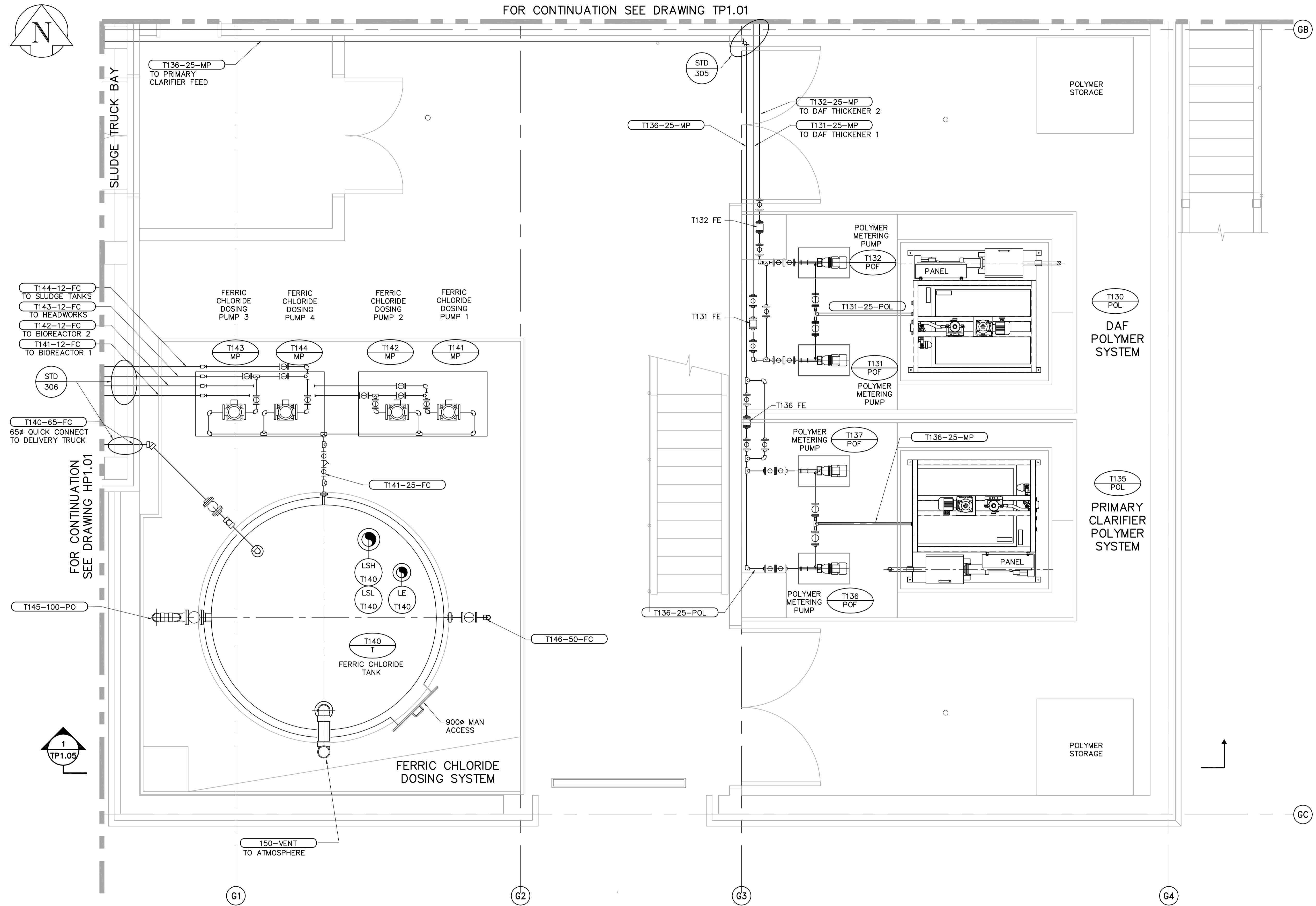
PLAN - POLYMER / FERRIC CHLORIDE SYSTEMS 1:25
