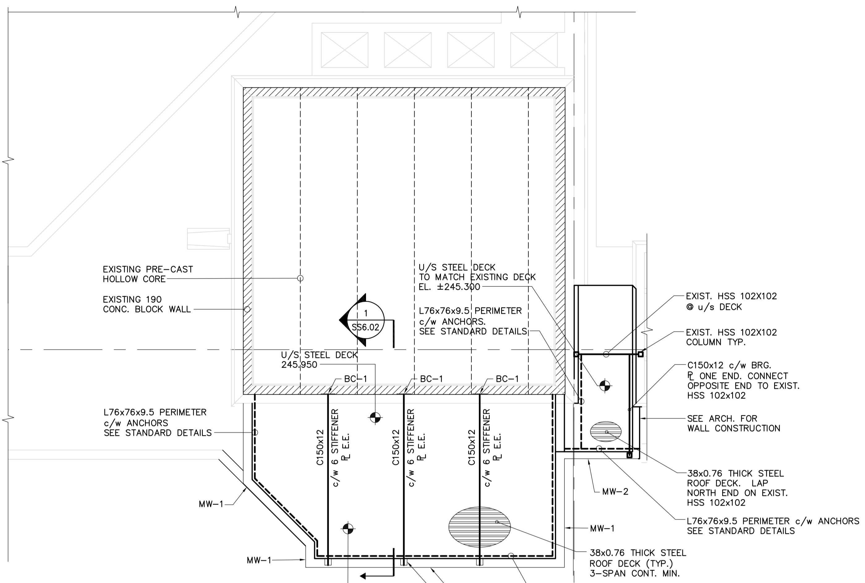
2 NEW ROOF PLAN SS6.01 SCALE 1:50
