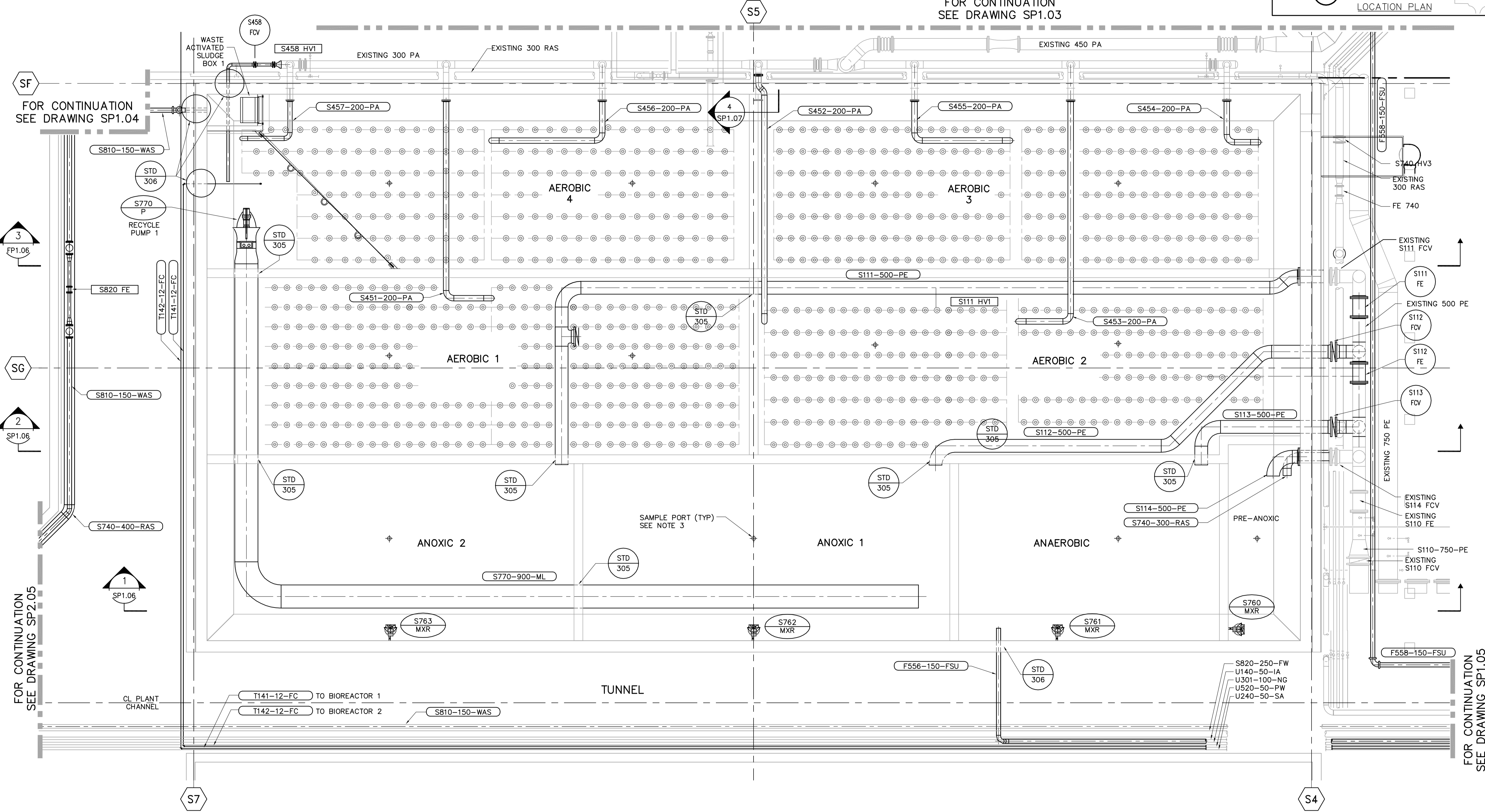
BIOREACTOR 1 - PLAN 1:75
