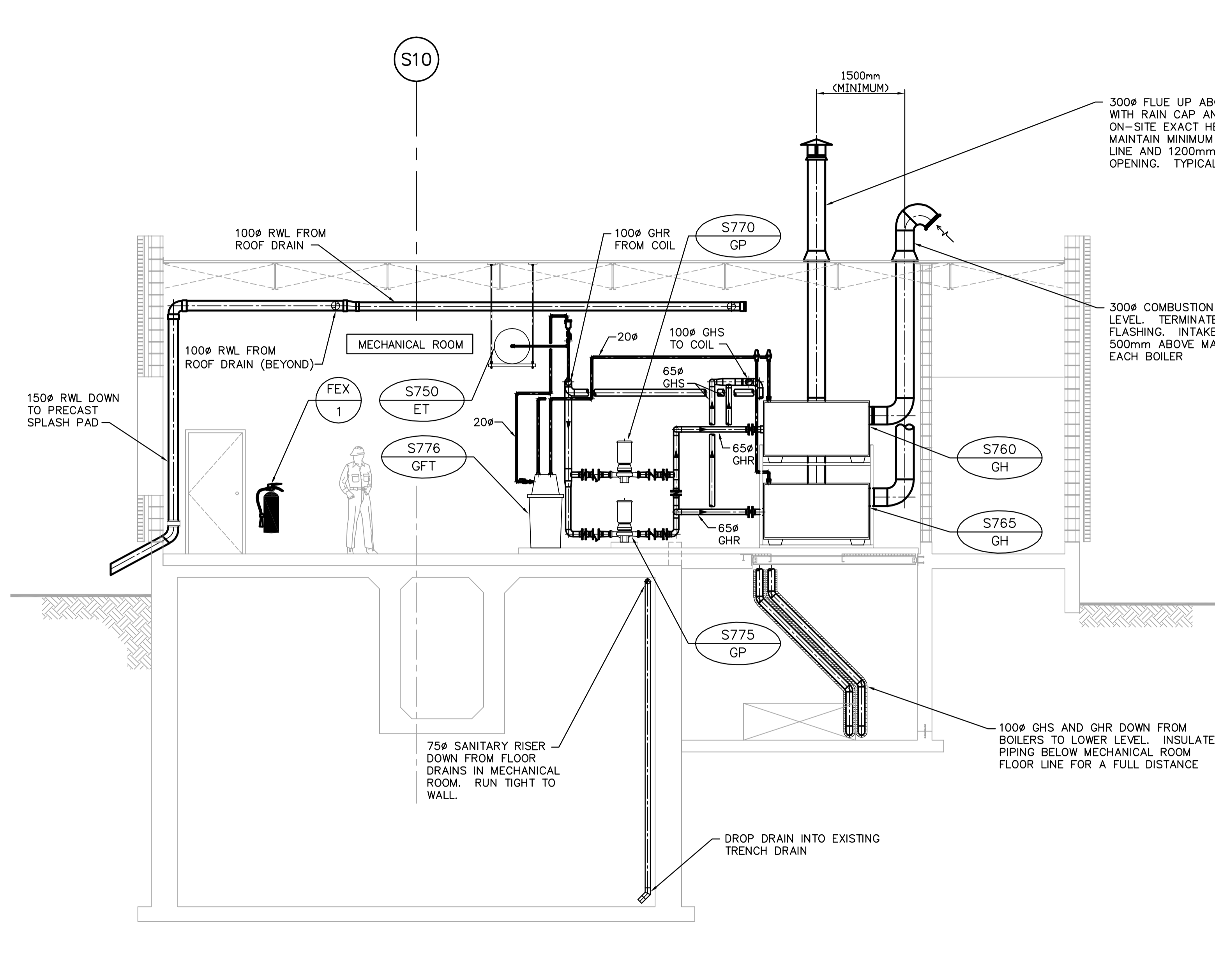
1 SECTION - MECHANICAL ROOM SM4.02 SCALE 1:50
