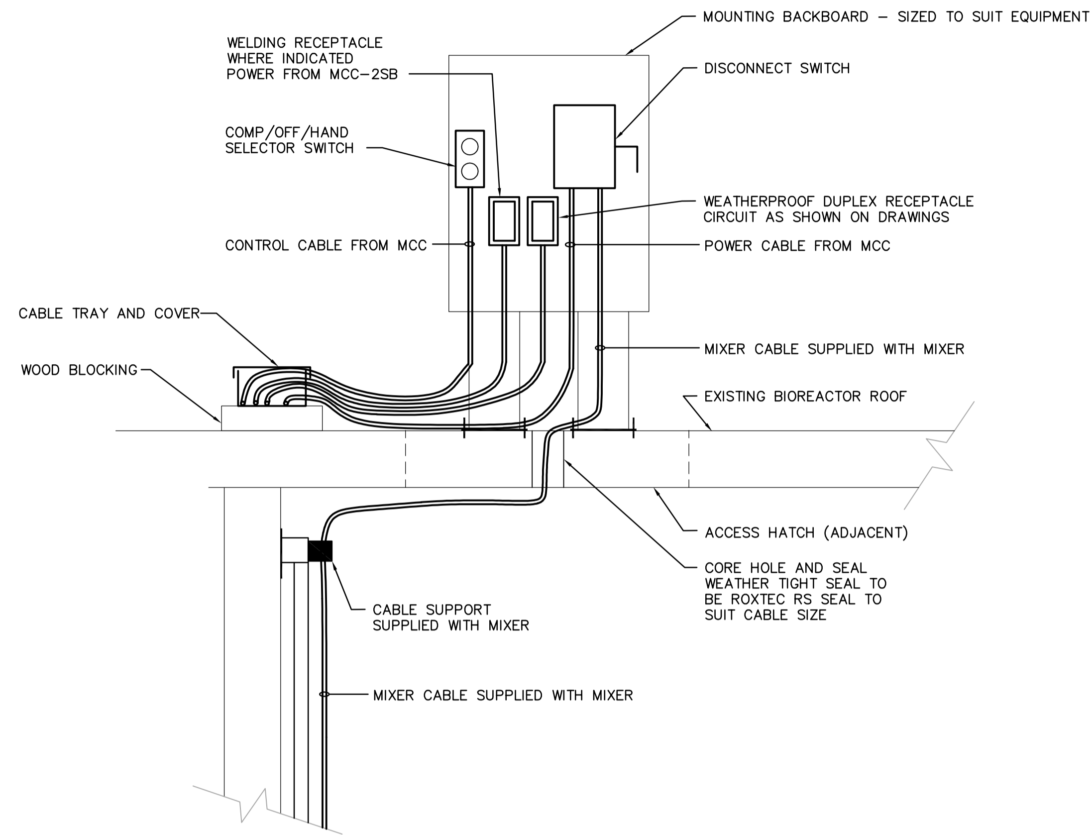
A DETAIL — BIOREACTOR ROOF MOTOR MOUNTING SE1.02 SCALE NTS SE1.03
