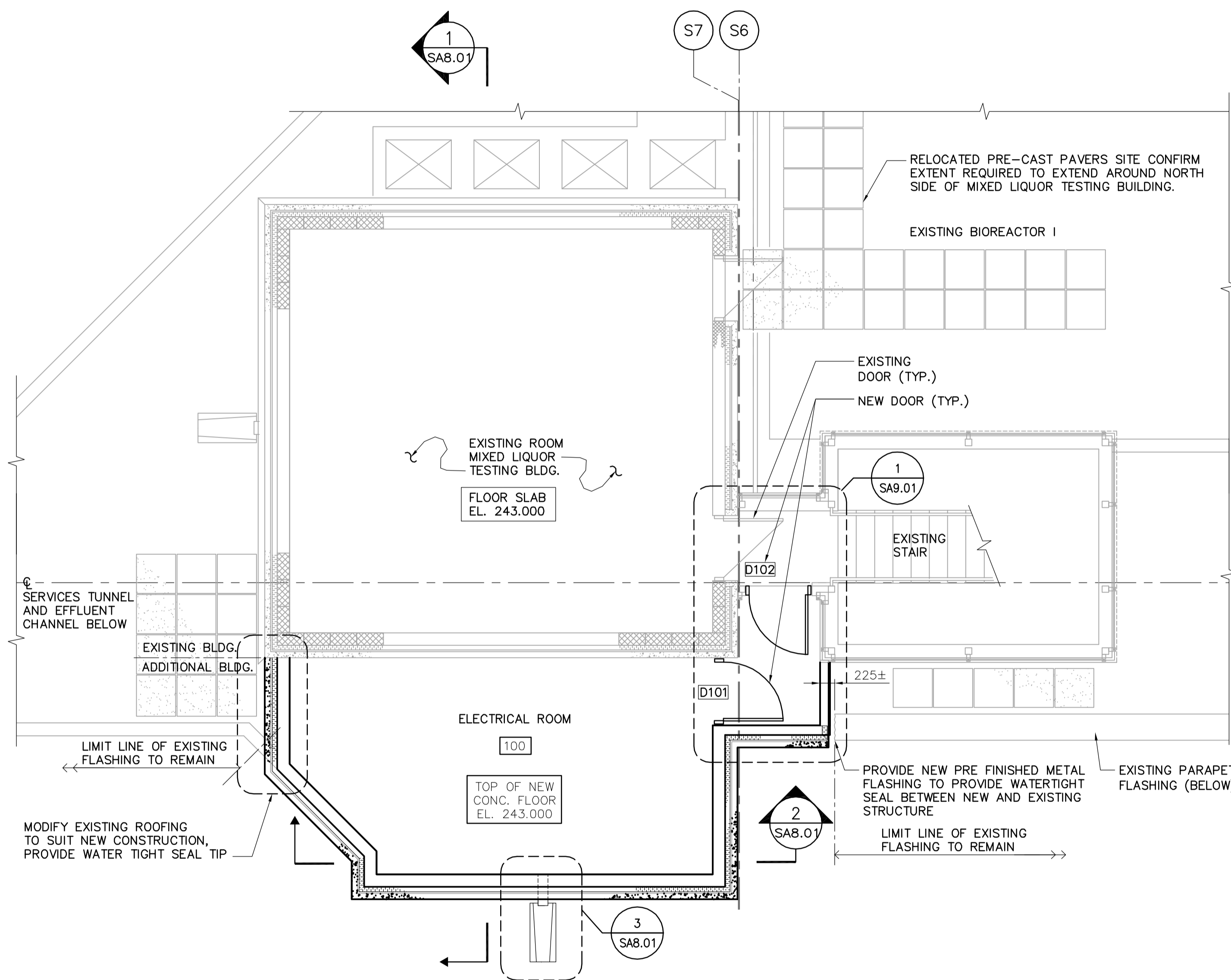
2 NEW MAIN FLOOR PLAN SA6.02 SCALE 1:50
