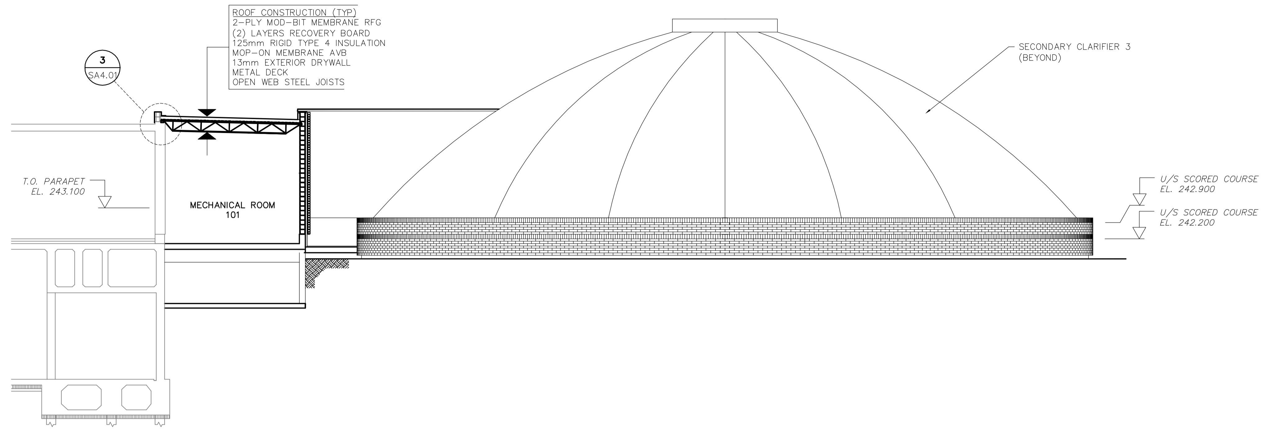
1 BUILDING SECTION SA1.01 1:100
