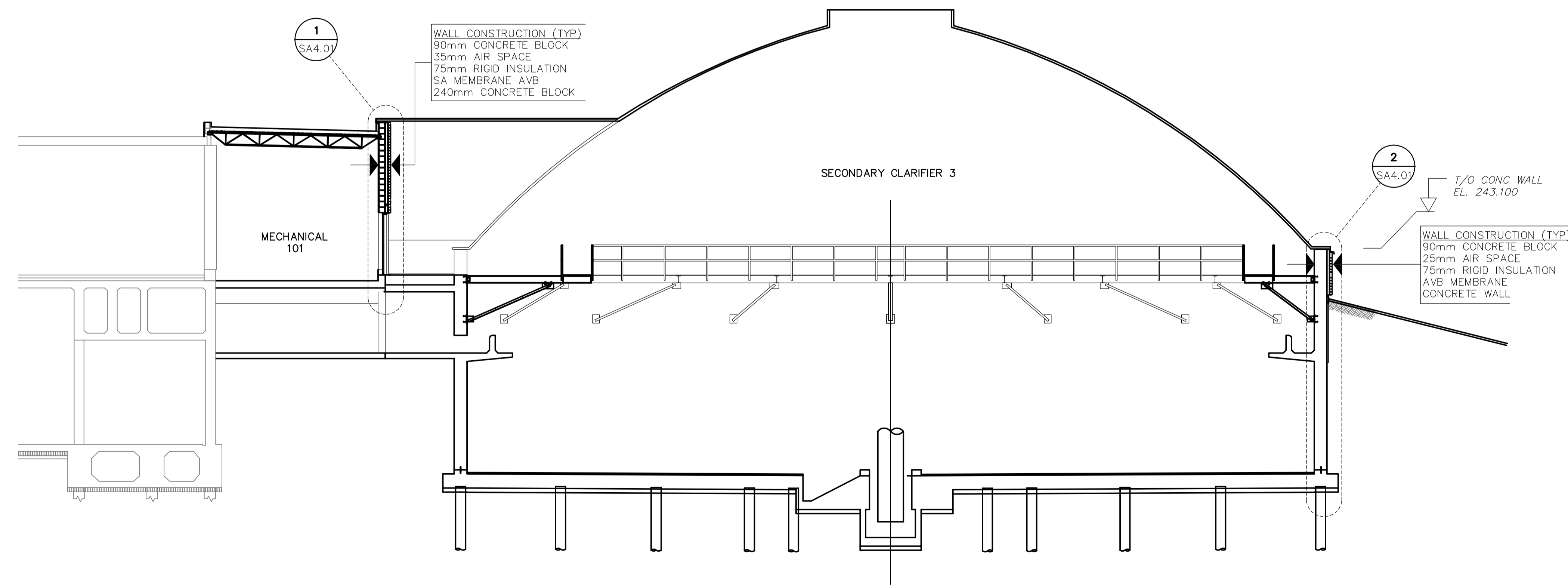
2 BUILDING SECTION SA1.01 1:100
