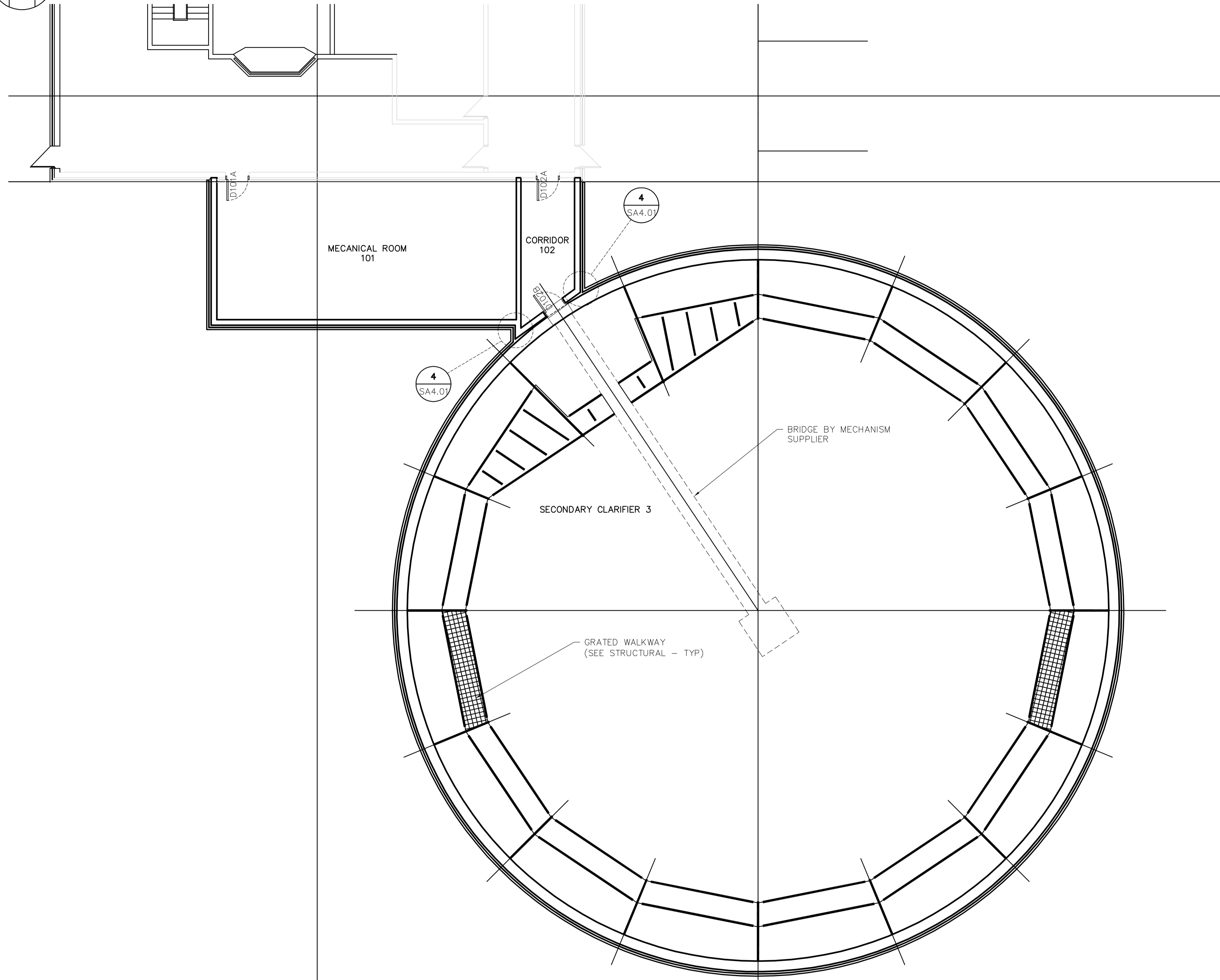
1 FLOOR PLAN SA1.02 1:100
