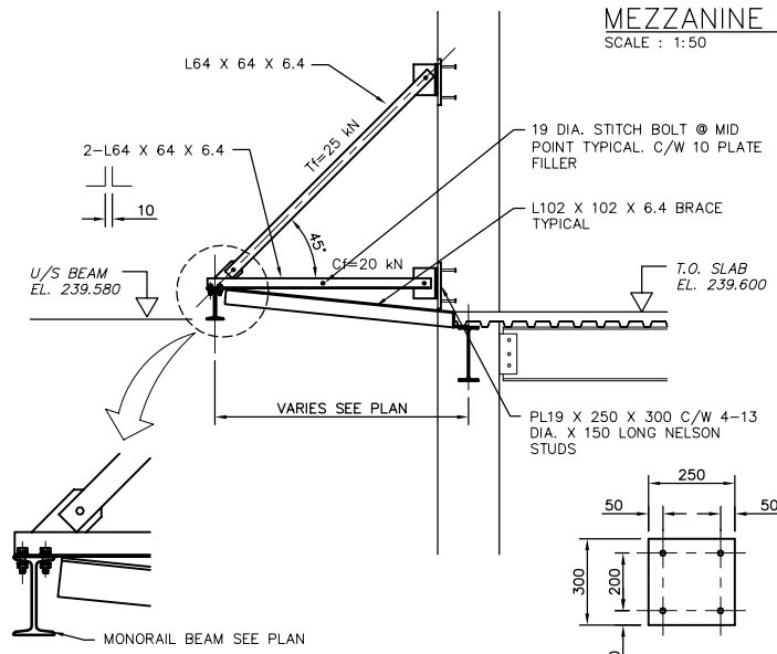
B MONORAIL SUPPORT DETAIL FS2.04 1:25
