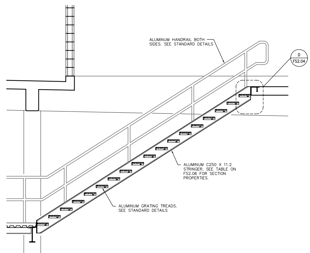
C STAIR SECTION FS2.04 1:25
