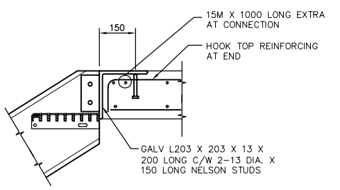
D DETAIL FS2.04 1:10
