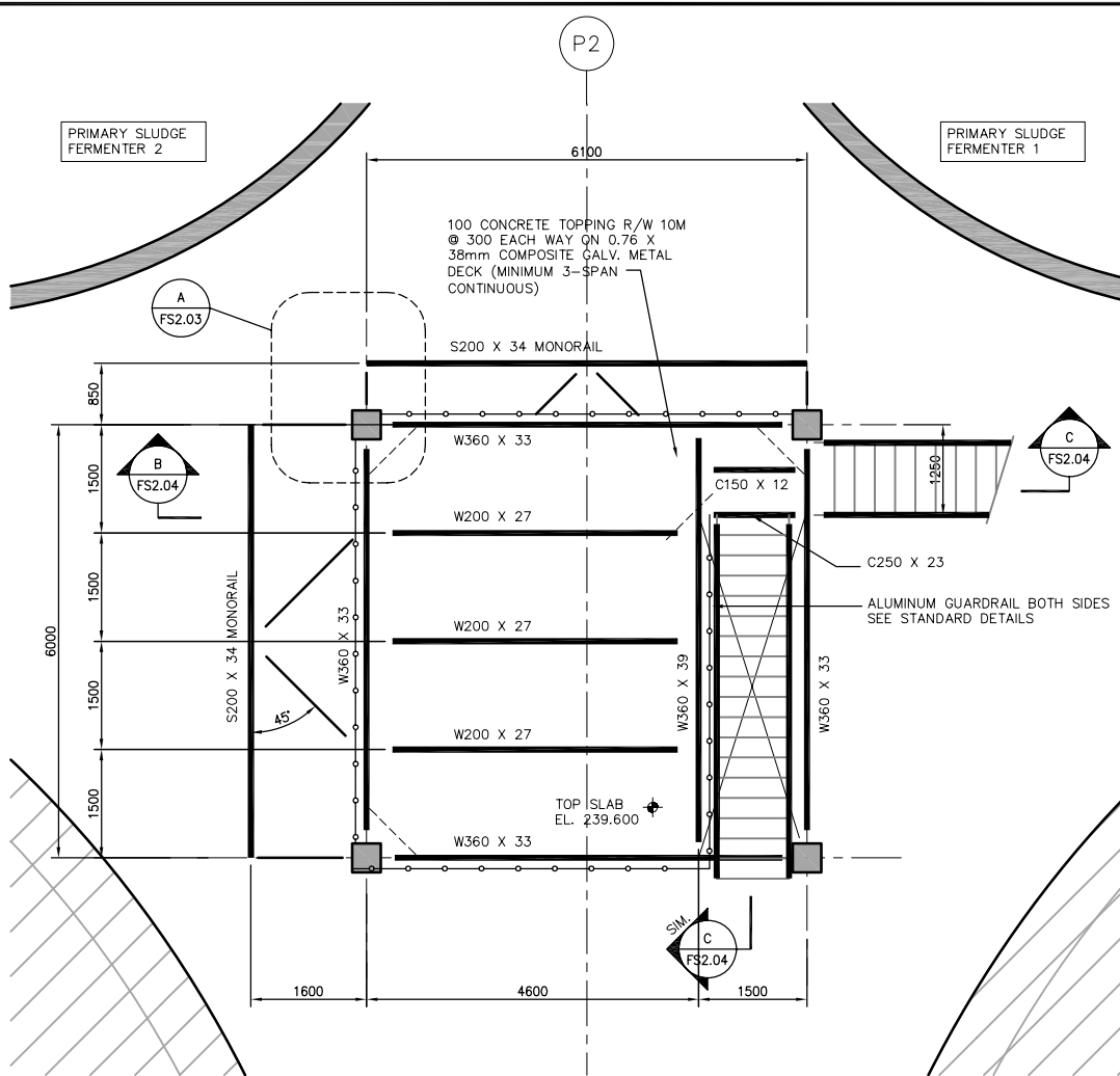
MEZZANINE FRAMING PLAN @ EL. 239.600 TOC SCALE: 1:50
