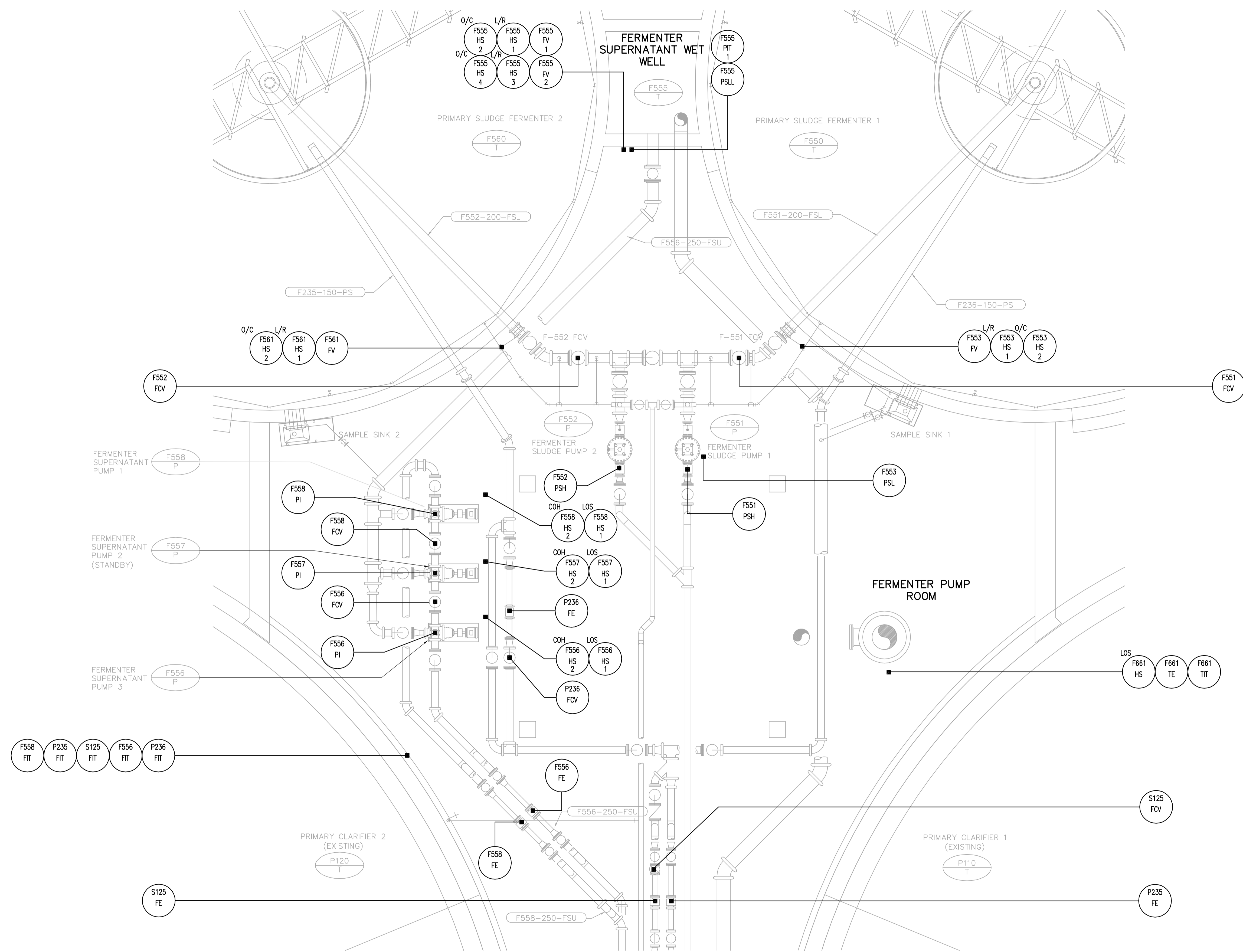
LOCATION PLAN - FERMENTER PUMP ROOM 1:50
