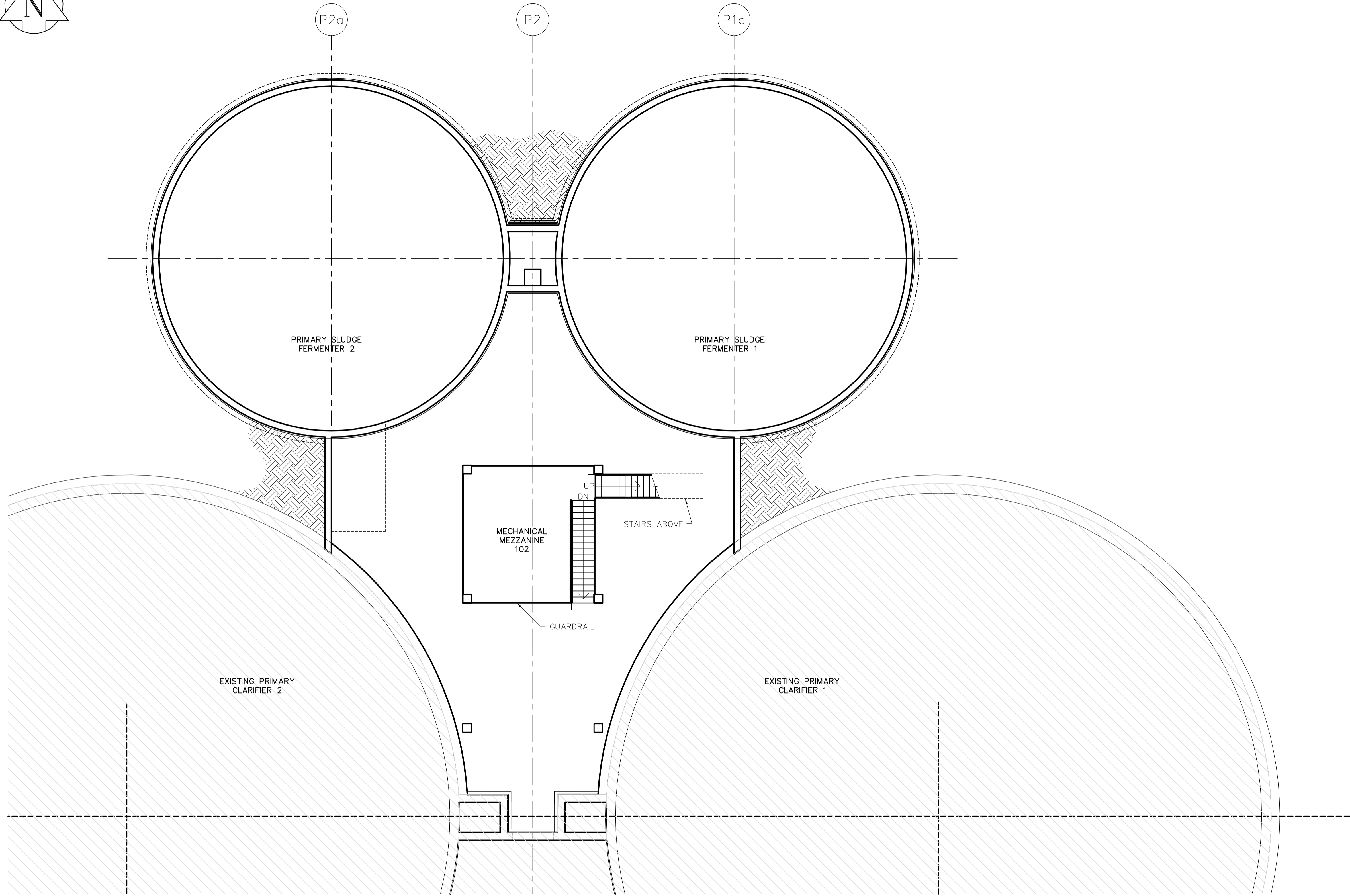
1 MEZZANINE PLAN FA1.03 1:100
