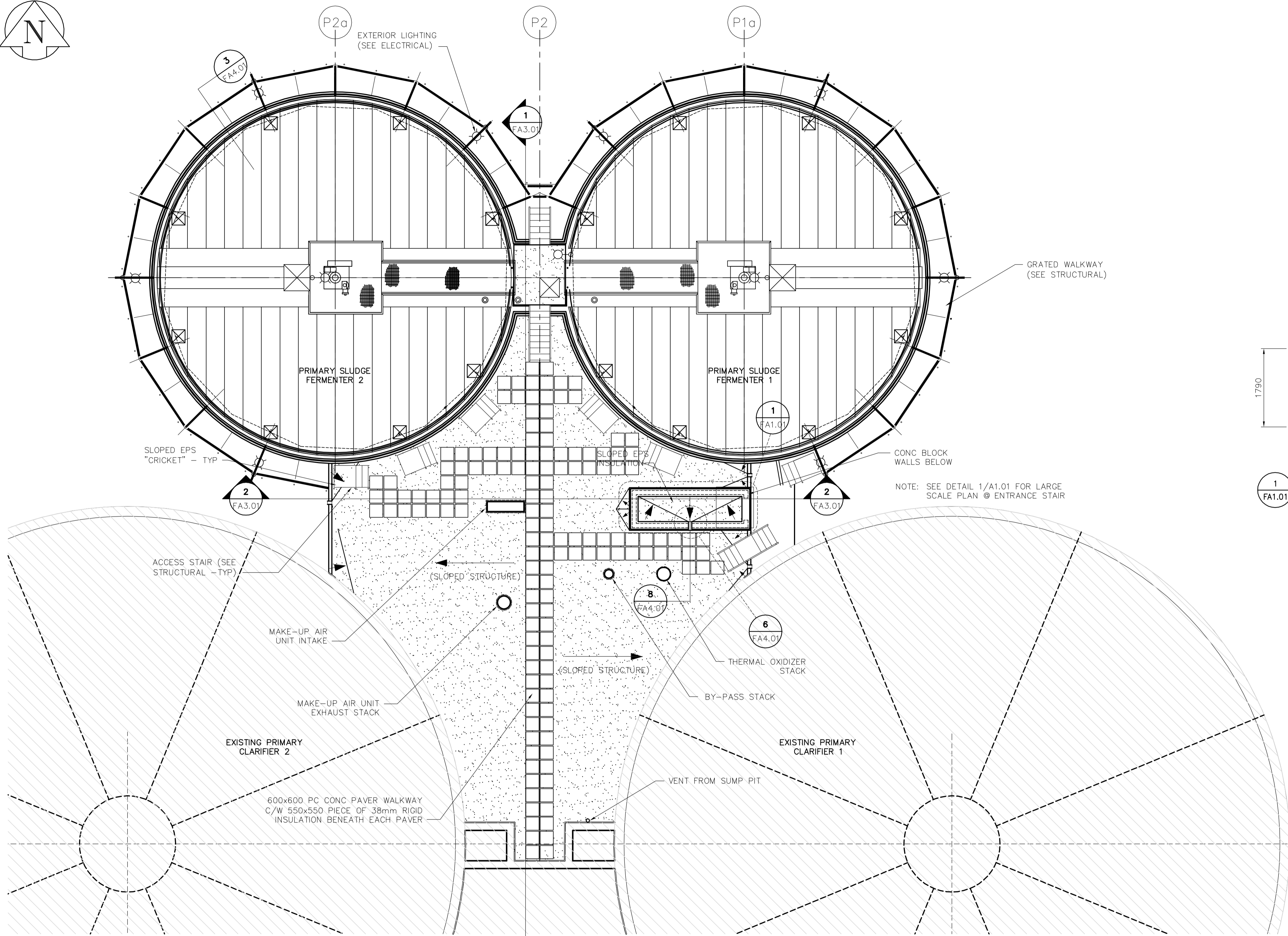
1 ROOF PLAN FA1.01 1:100
