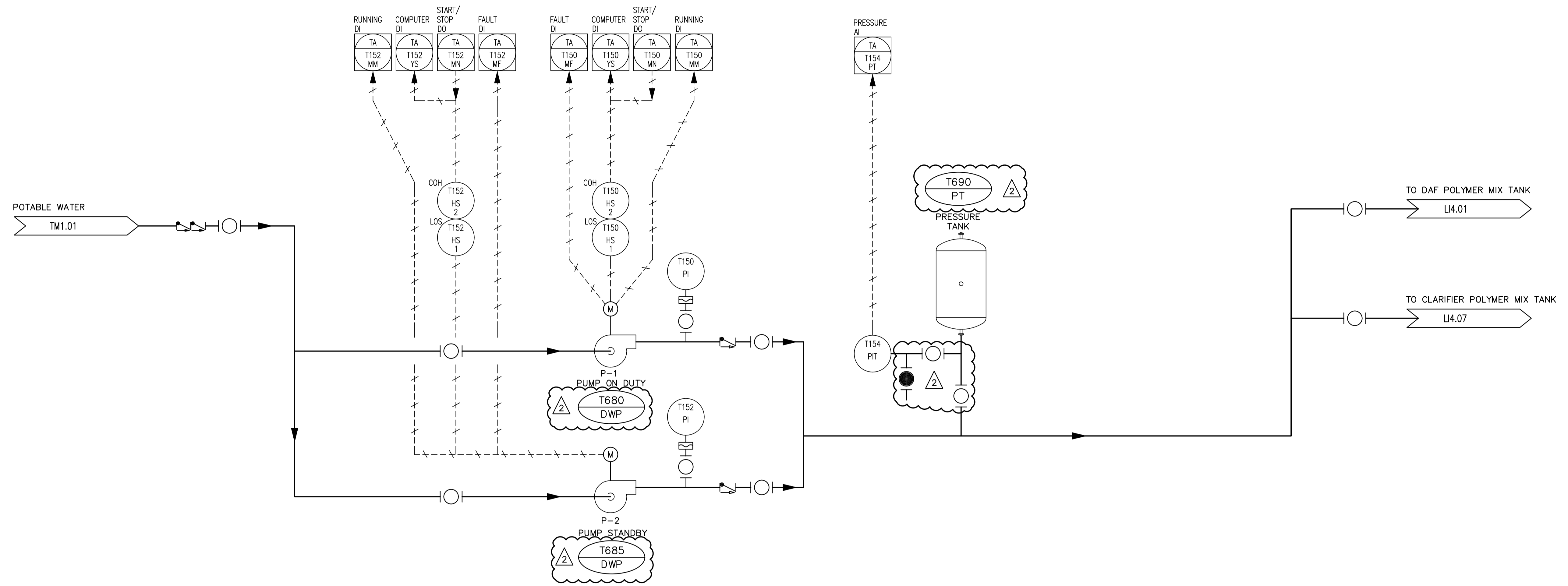
1 POLYMER WATER SUPPLY SCHEMATIC LM4.09 SCALE NTS
