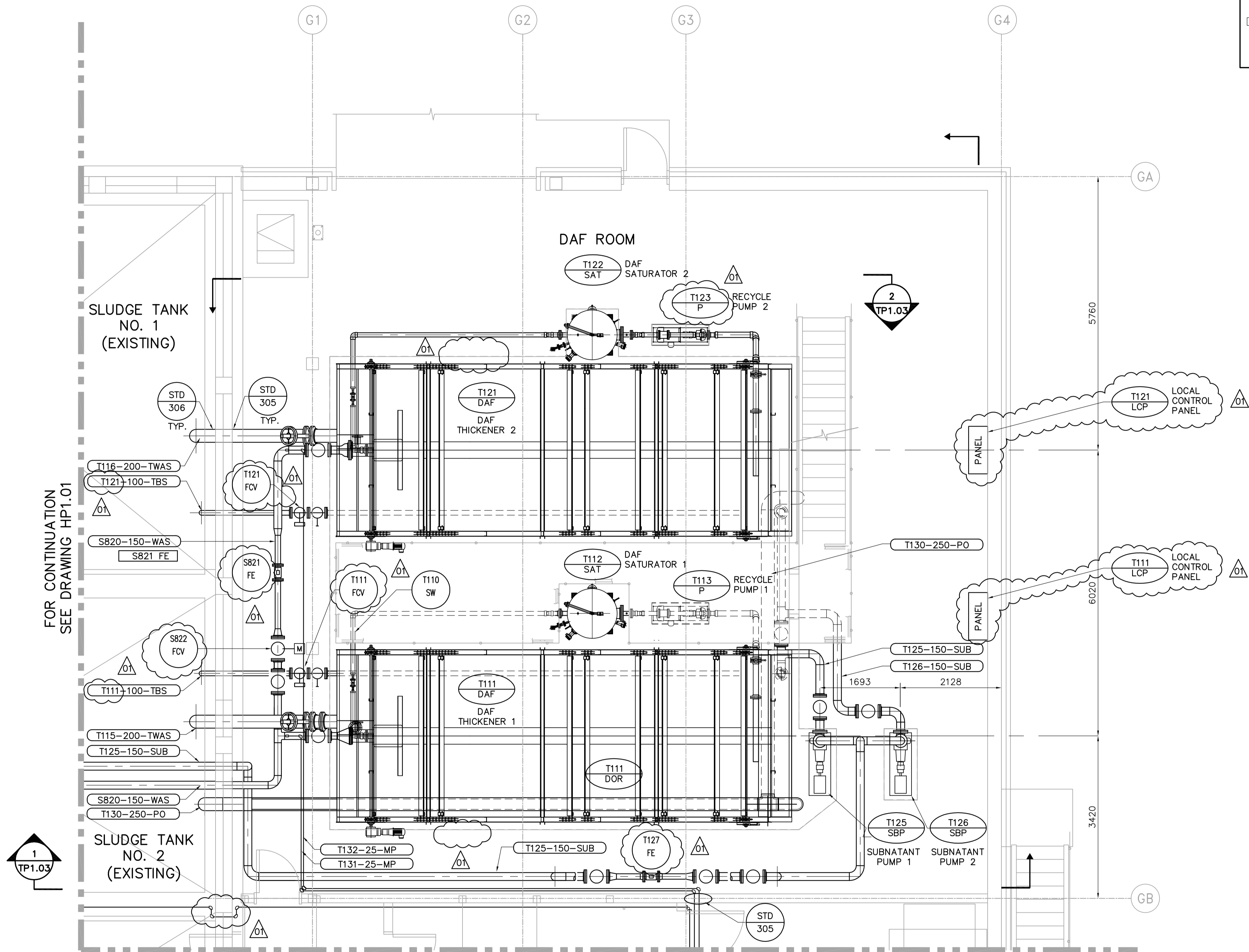
PLAN - DAF BUILDING 1:50
