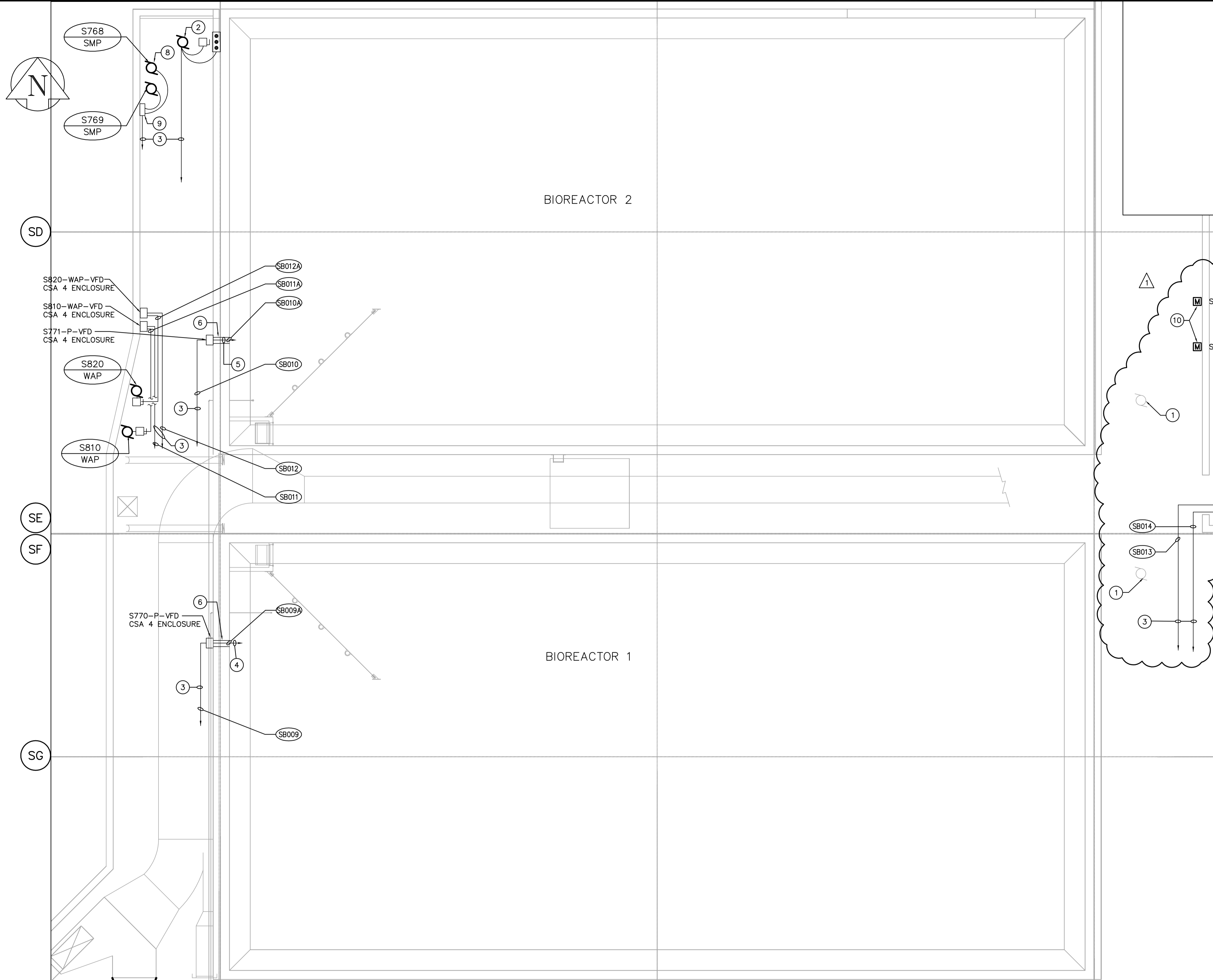
BIOREACTORS 1 & 2 - LOWER LEVEL POWER PLAN SCALE: 1:100
