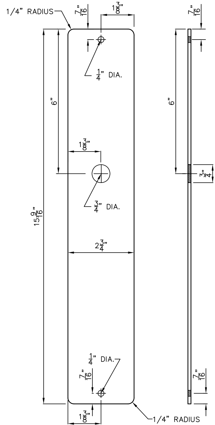
③ AUDIBLE BOX BACK PLATE FRONT & SIDE VIEW
