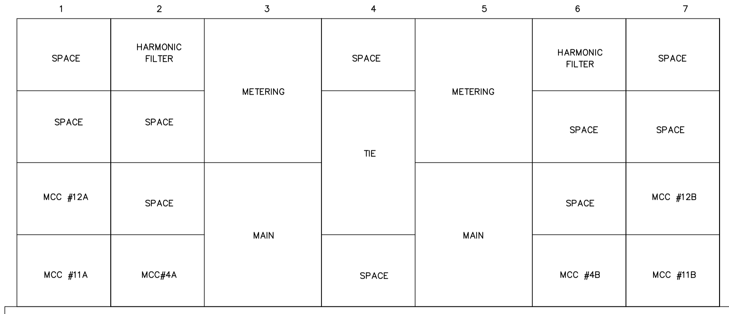
SWITCHGEAR #2A, #2B ELEVATION (NOT TO SCALE)
