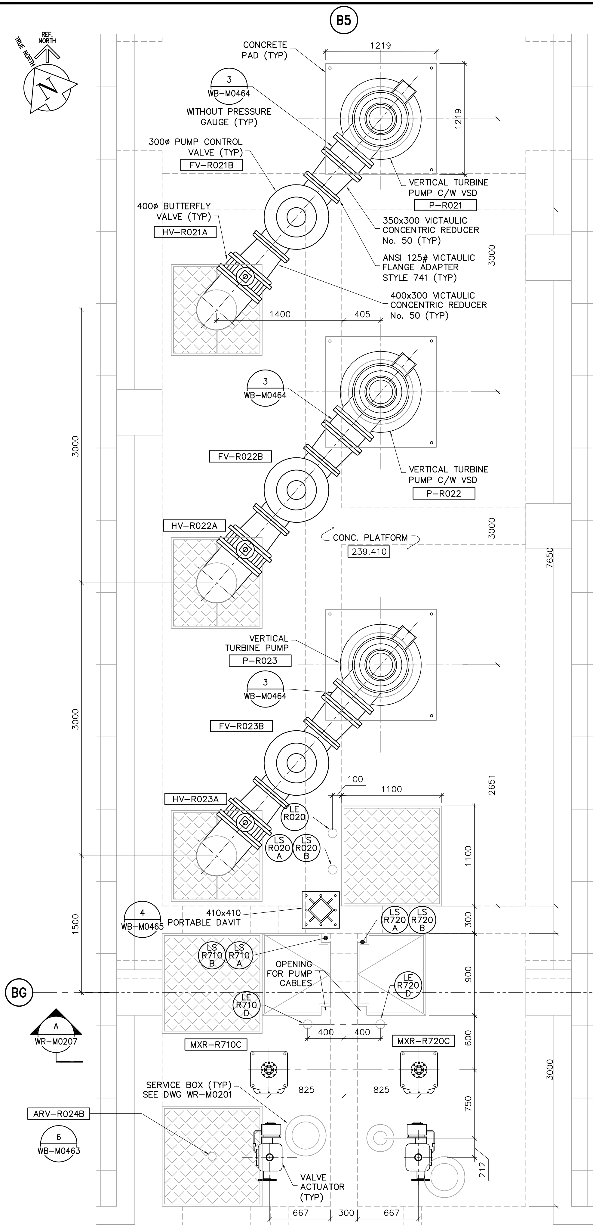
PLAN AT ELEVATION 239.410 WR-M0121 1:25
