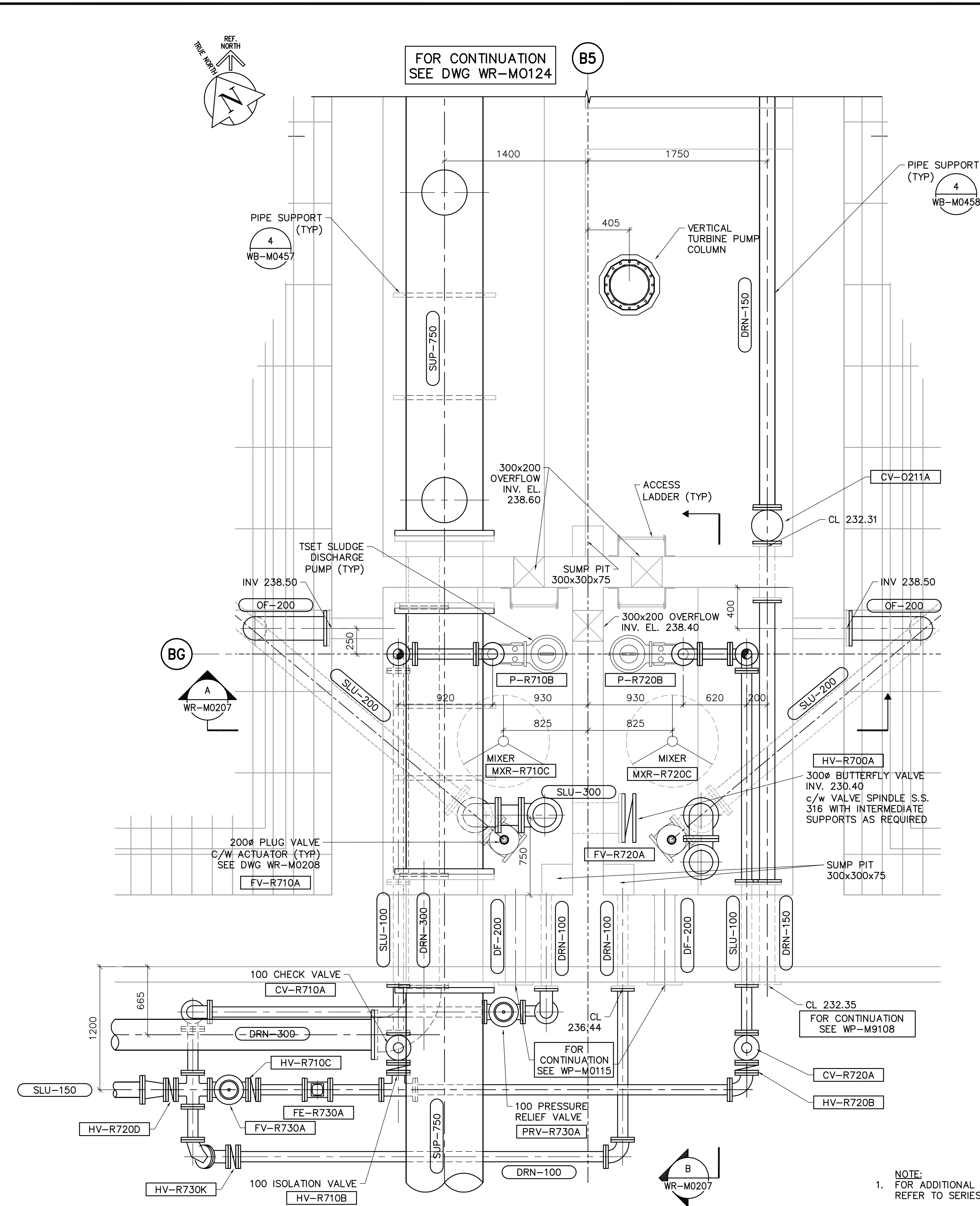
PLAN AT ELEVATION 239.000 WR-M0111 1:25
