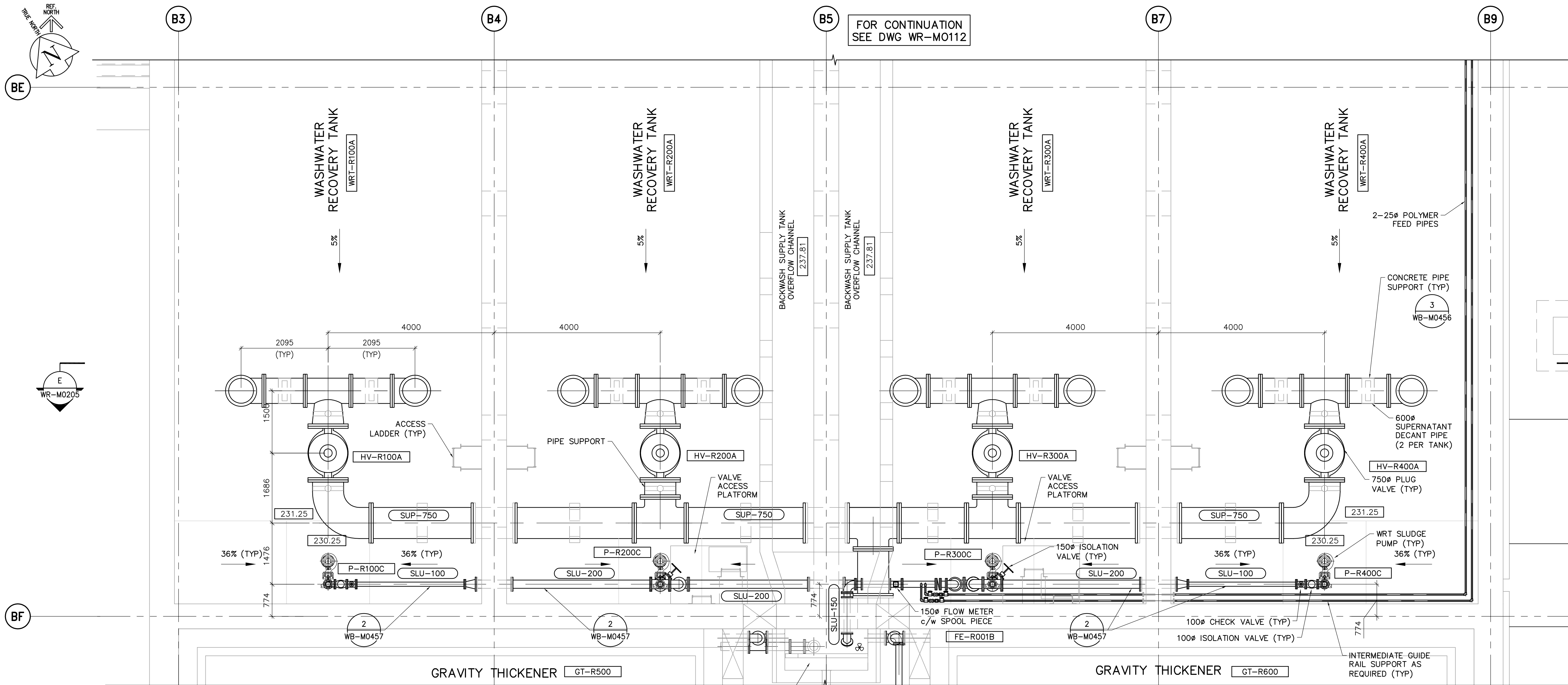
PLAN AT ELEVATION 239.000 WR-M0111 1:50
