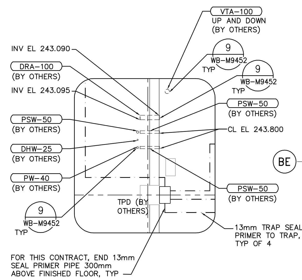
1 DETAIL 1:50
