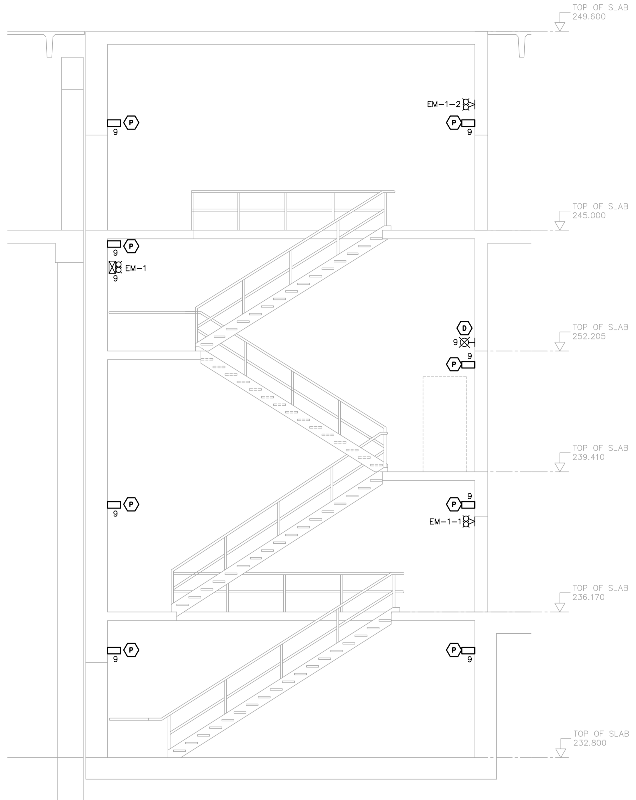
STAIRWELL NO.9 – LIGHTING
