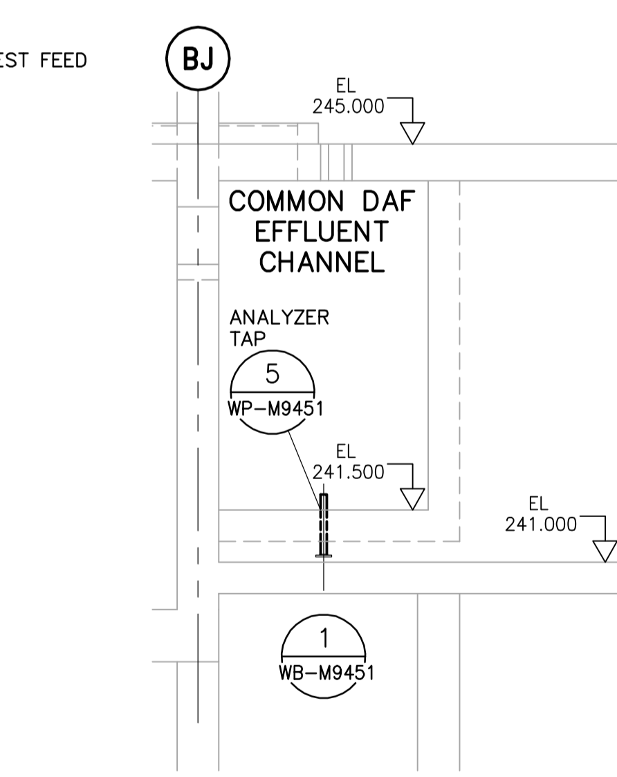
Q SECTION - EMBEDDED ANALYSER TAP TYP. 2 WP-M9101 1:50
