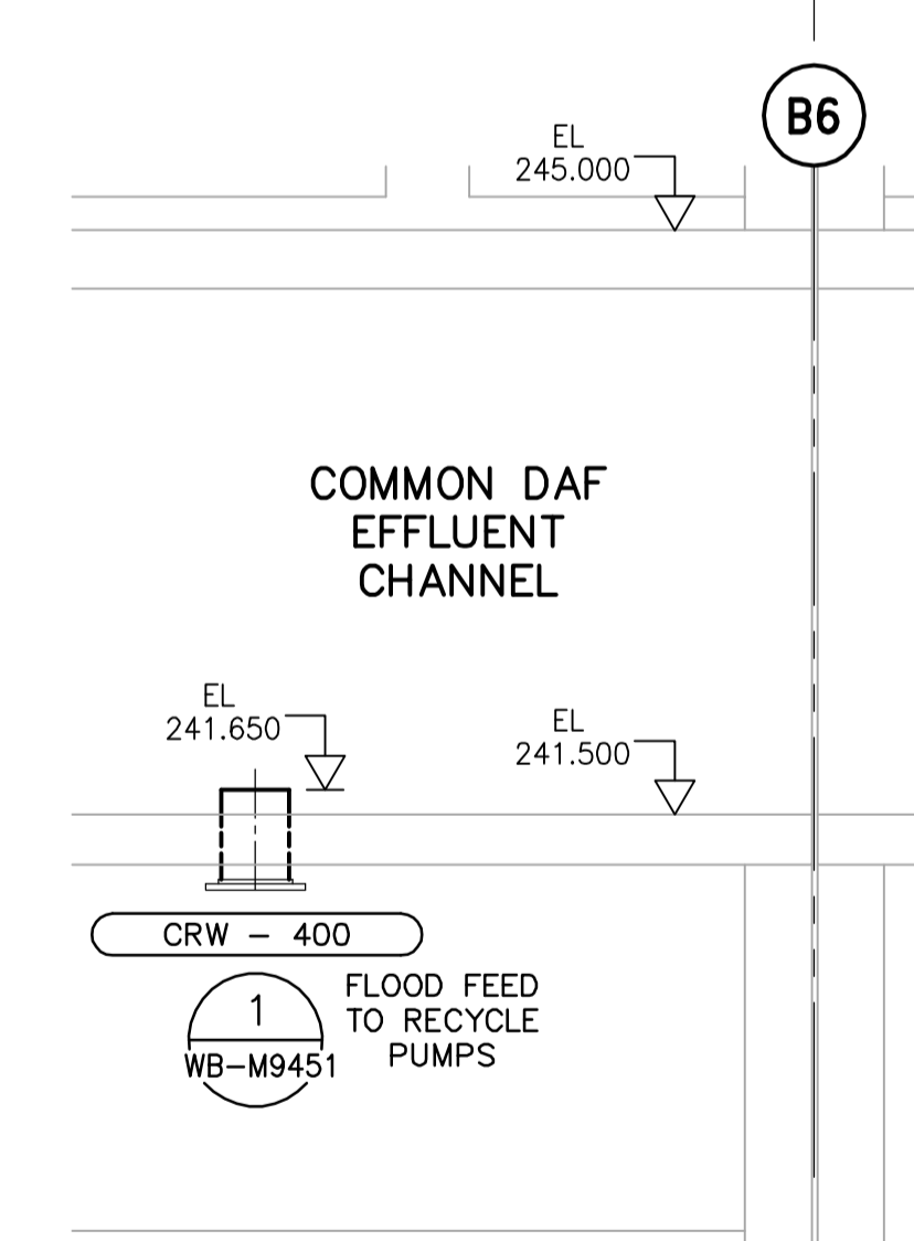
D SECTION - FEEDS TO RECYCLE PUMPS - TYP. 2 WP-M9101 1:50
