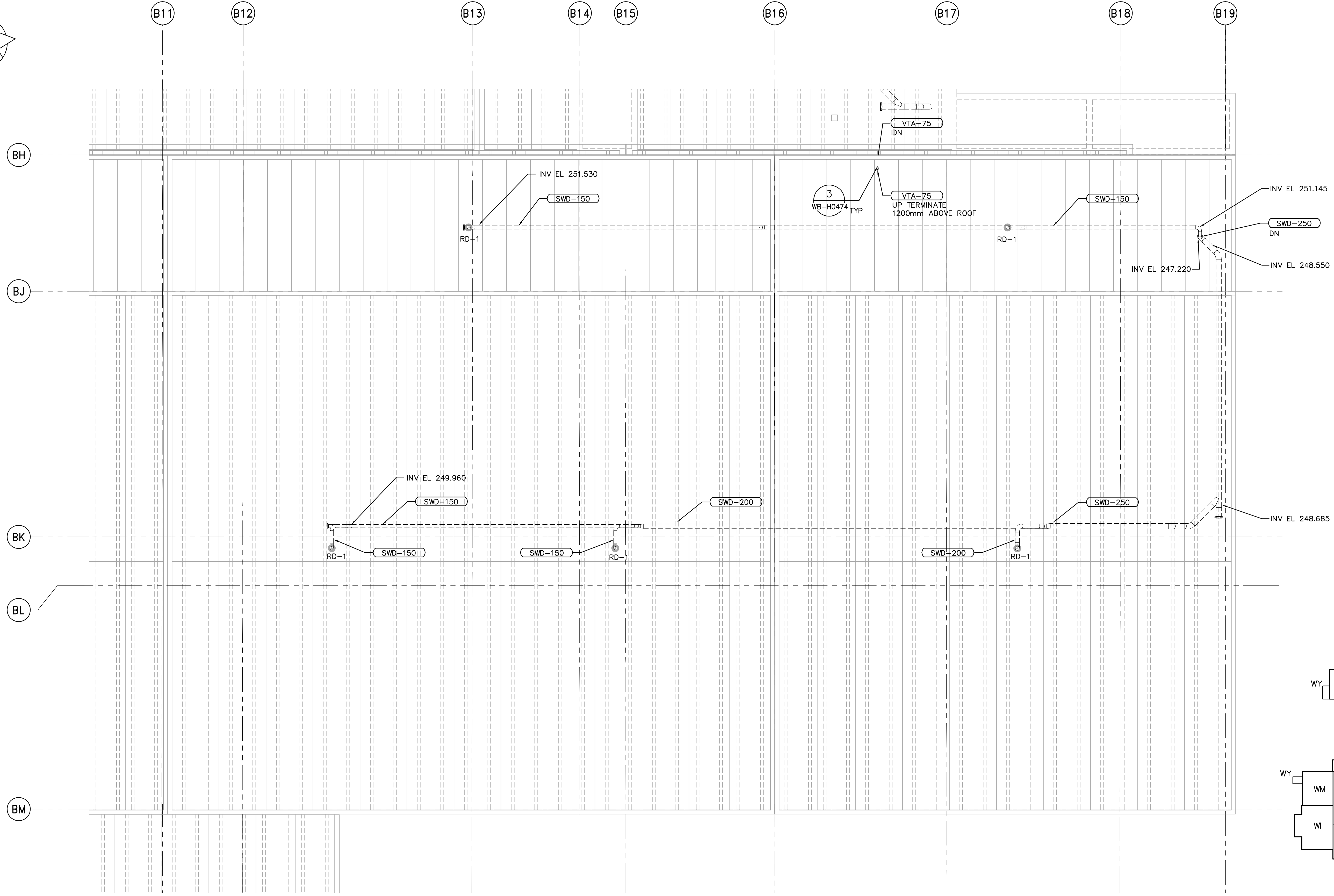
ROOF PLAN 1:100
