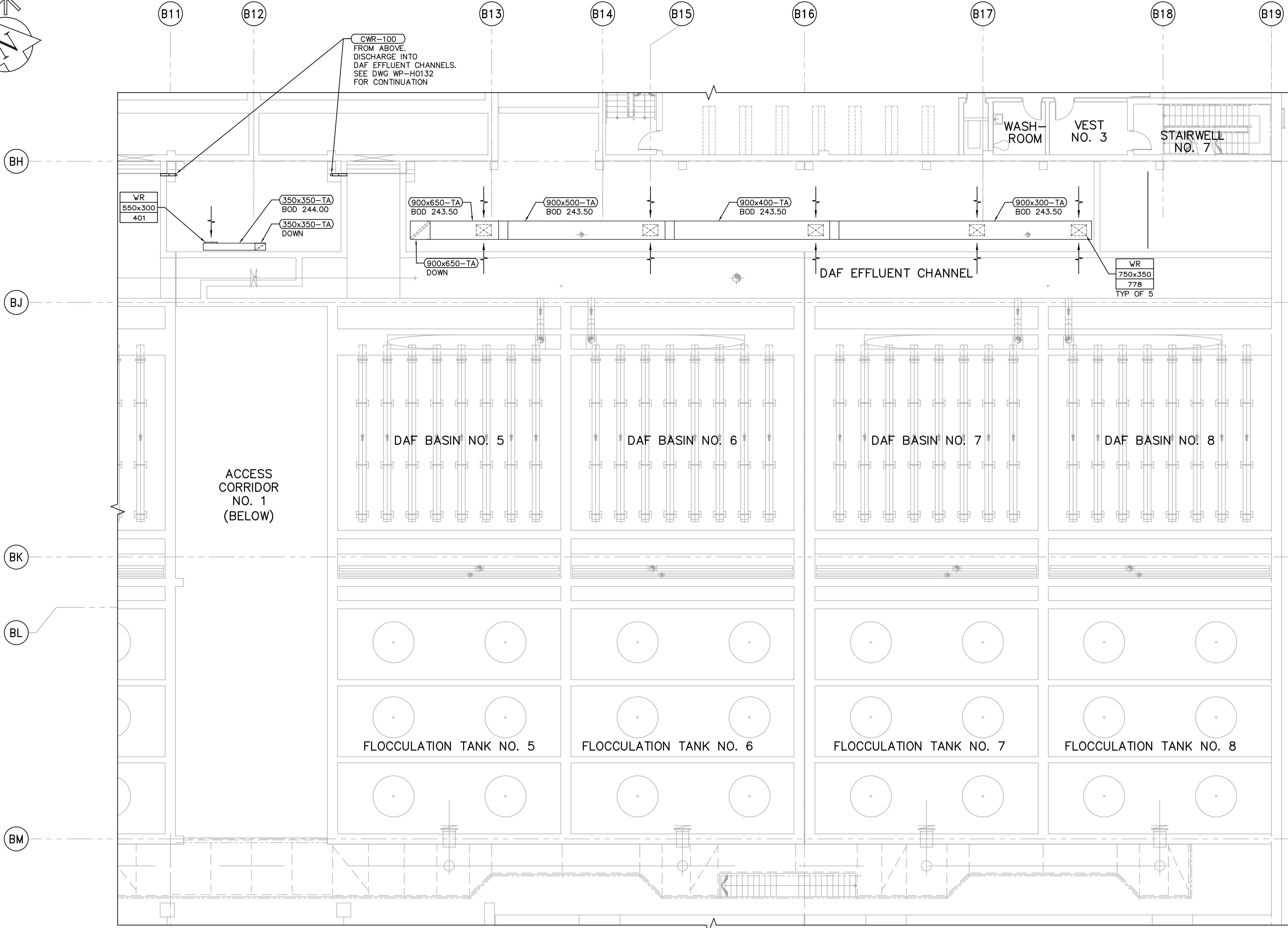
SECOND FLOOR PLAN 1:100
