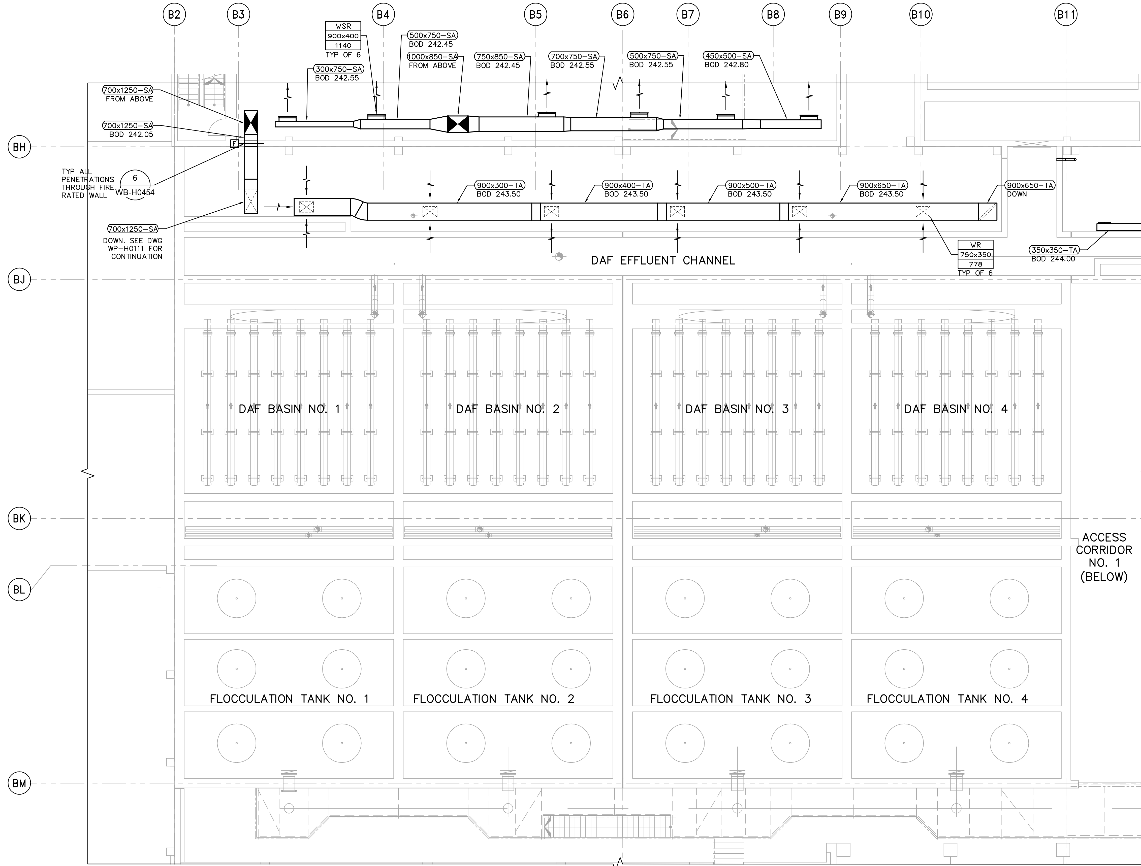
SECOND FLOOR PLAN 1:100
