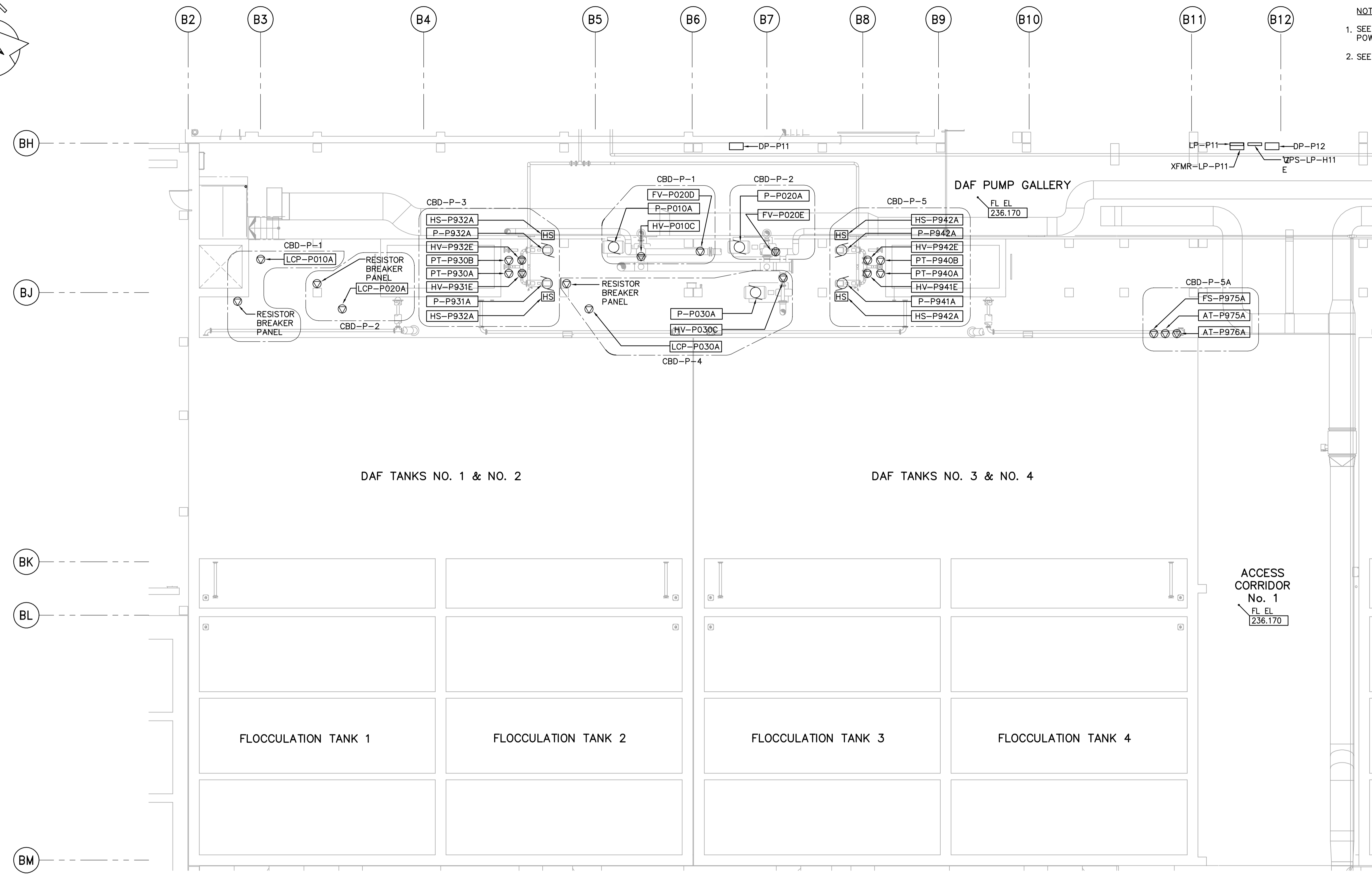
FIRST FLOOR PROCESS PLAN (AREA 1) 1:100
