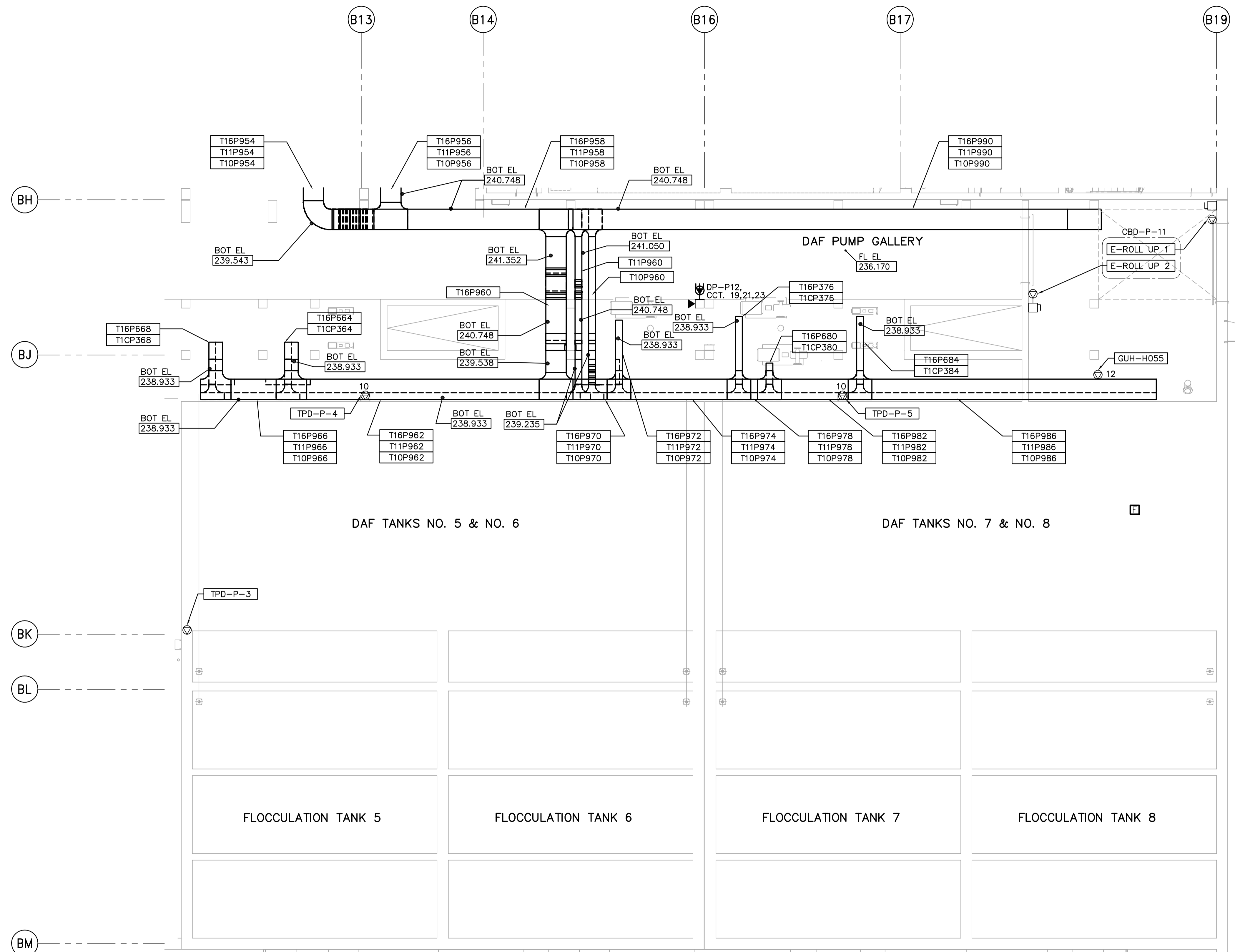
FIRST FLOOR FACILITY PLAN (AREA 2) 1:100
