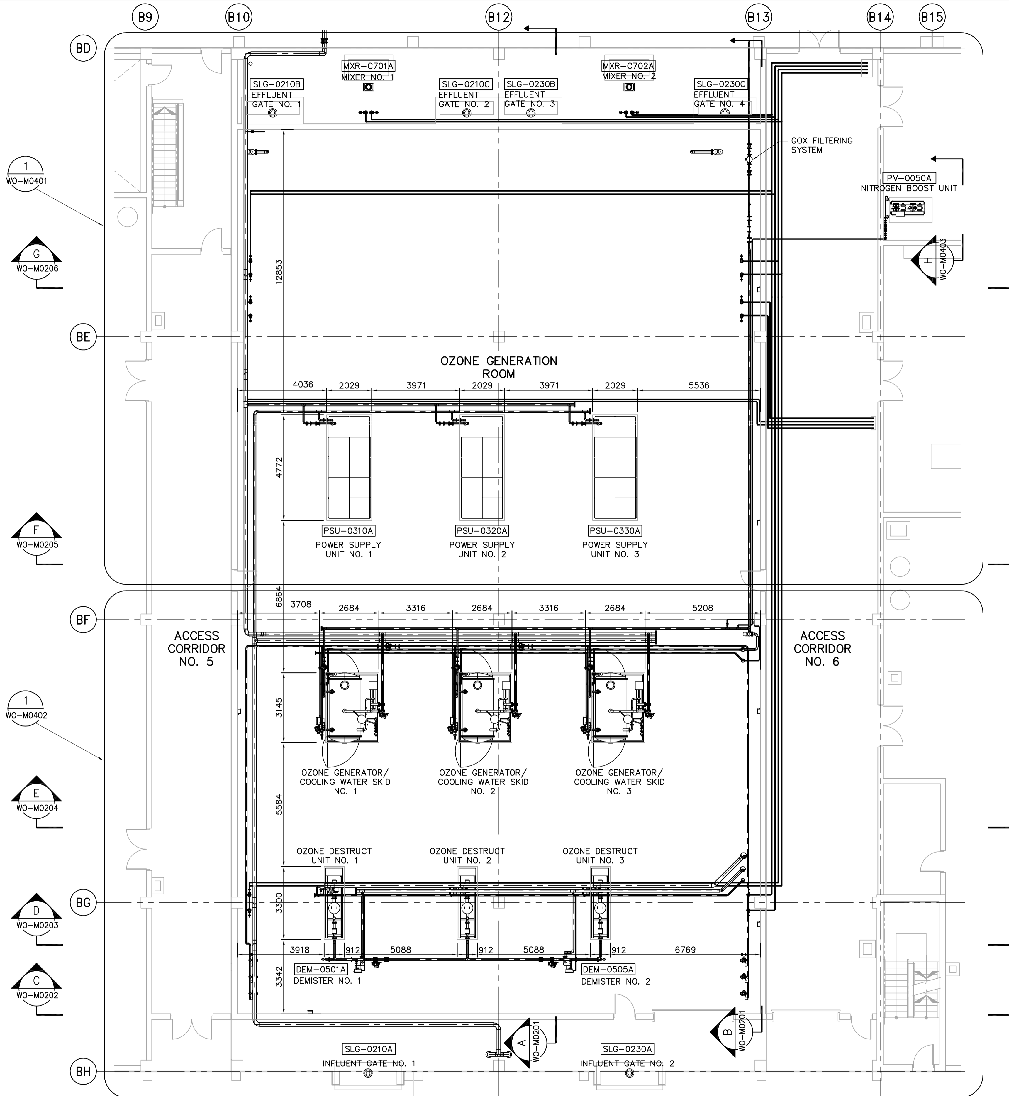
THIRD FLOOR PLAN 1:100
