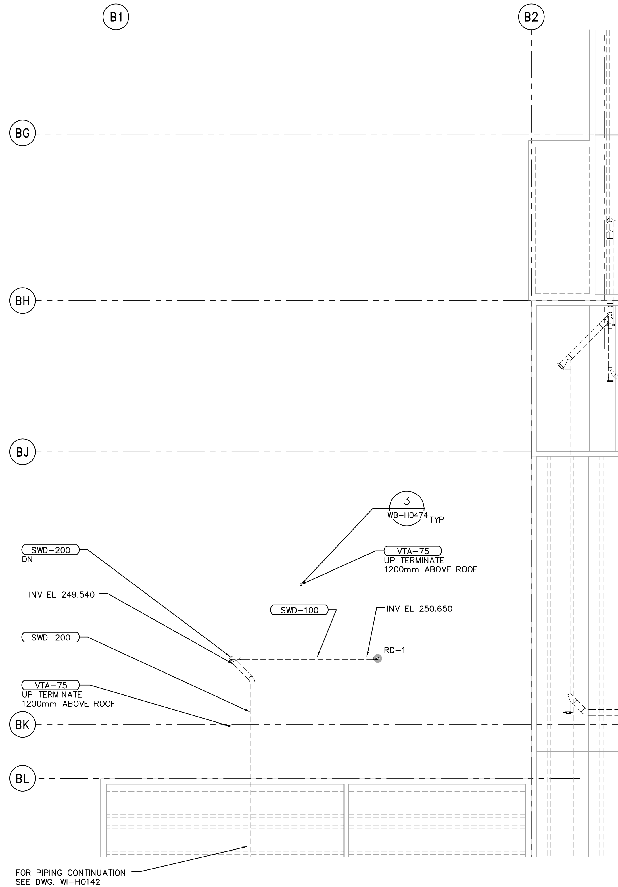
ROOF PLAN 1:100
