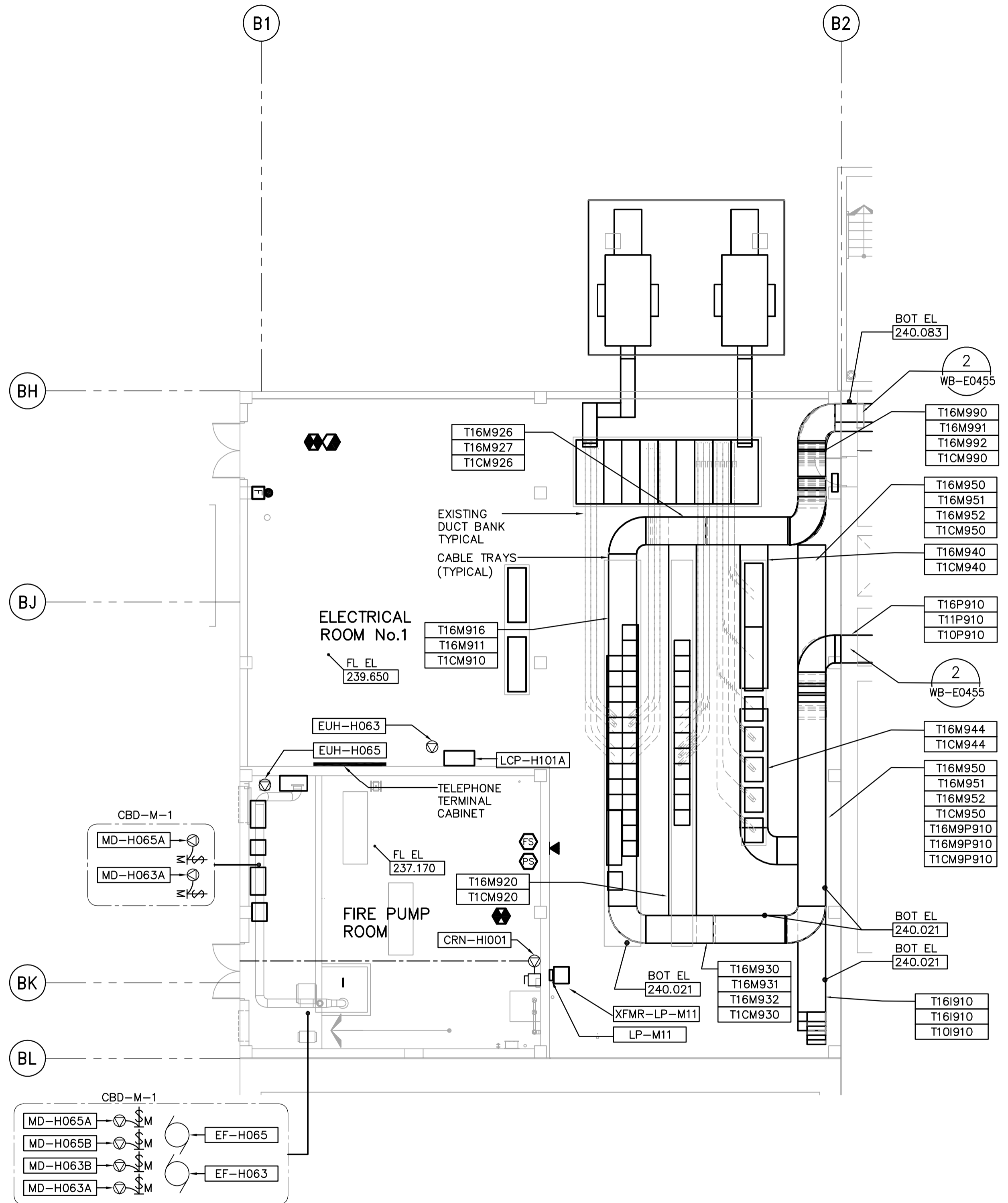
FIRST FLOOR FACILITY PLAN 1:100
