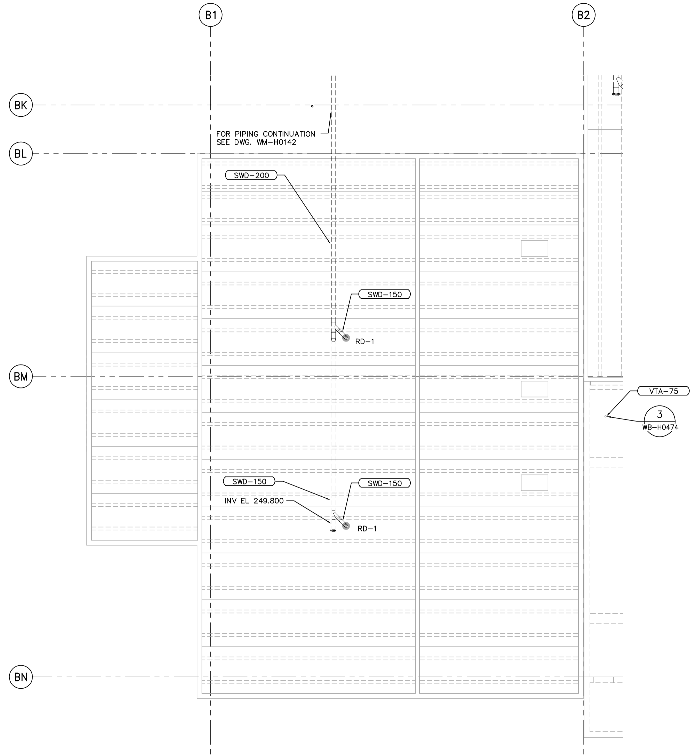
ROOF PLAN 1:100
