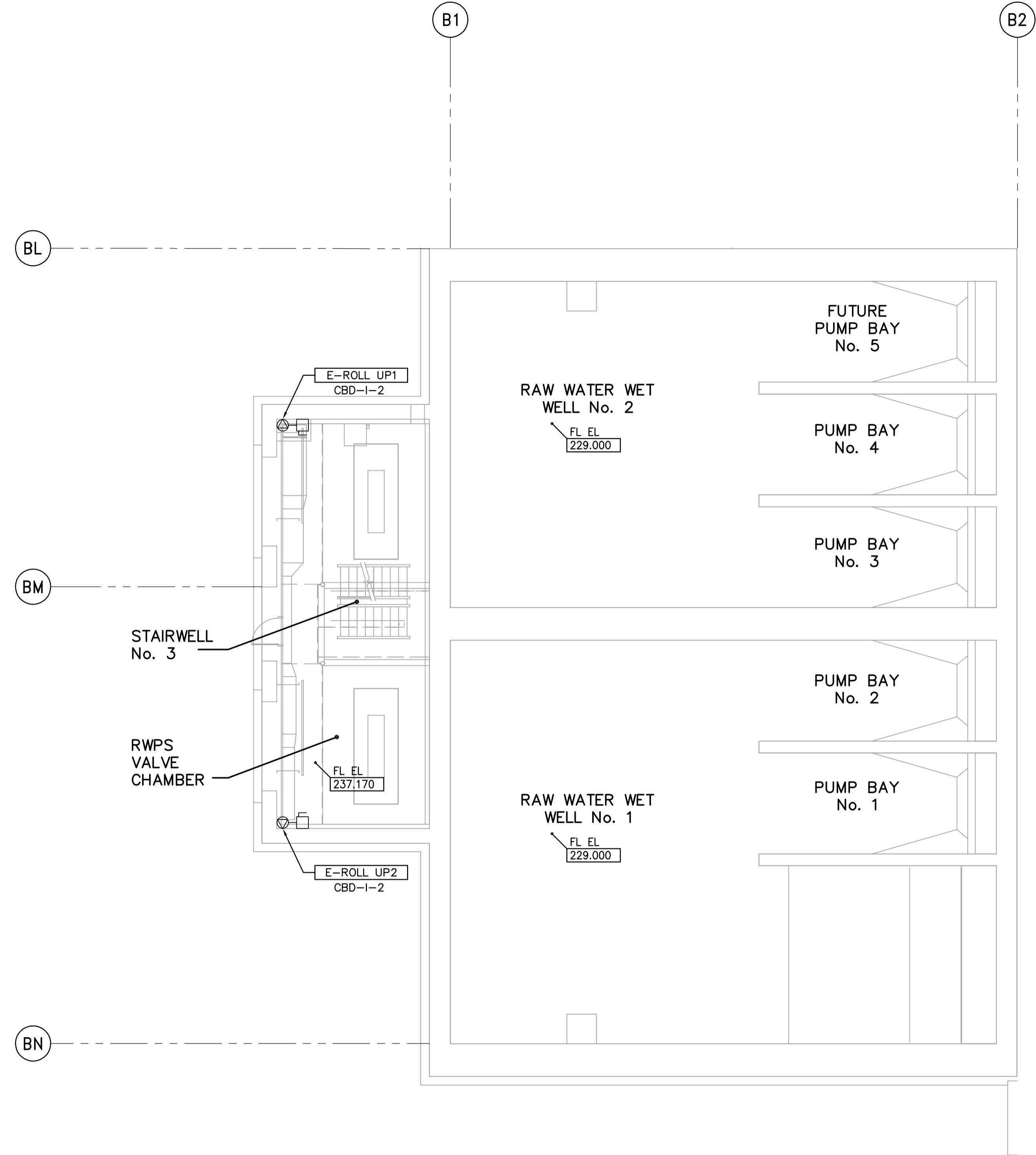
FIRST FLOOR FACILITY PLAN 1:100
