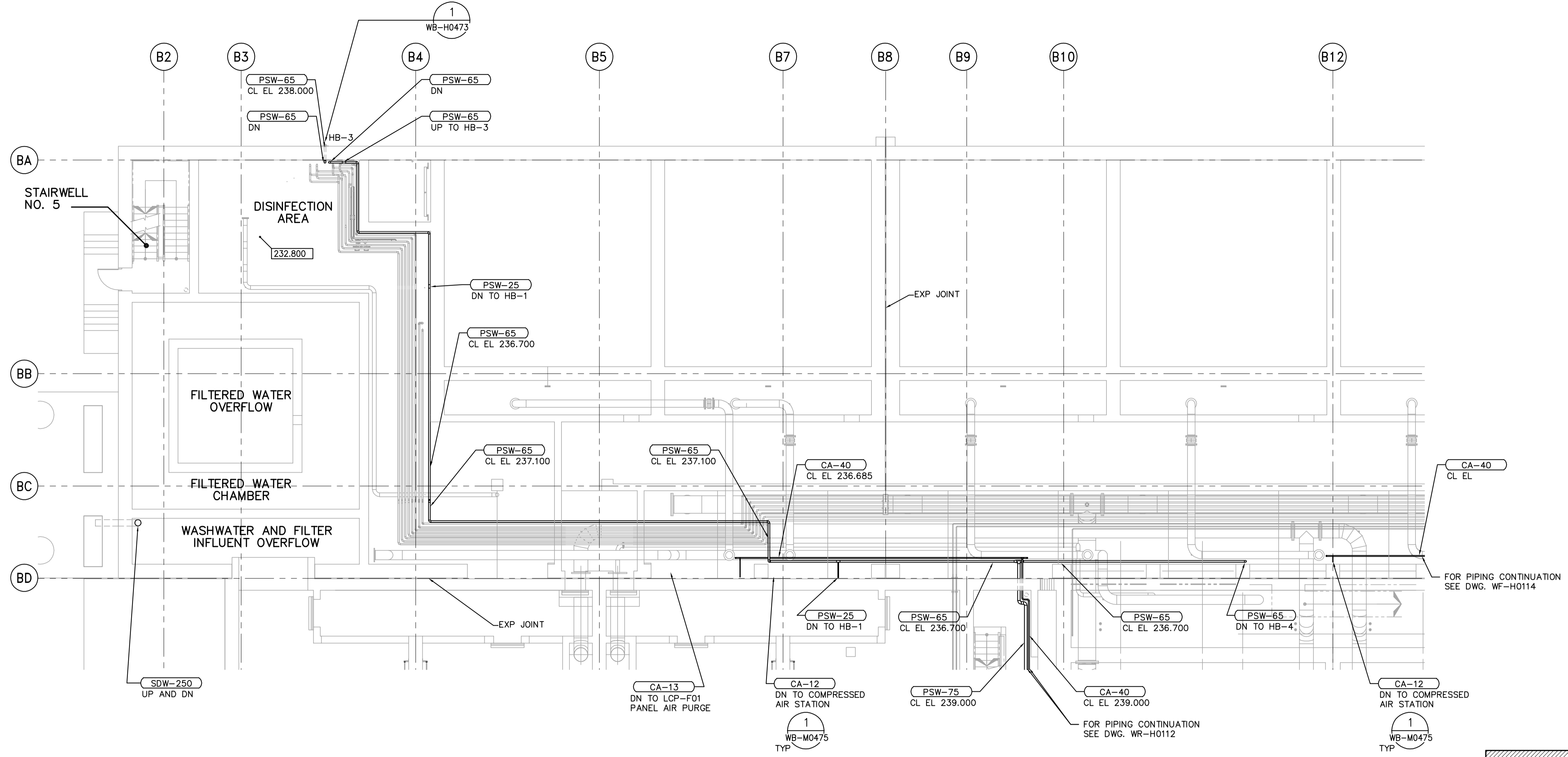
FIRST FLOOR PLAN 1:100
