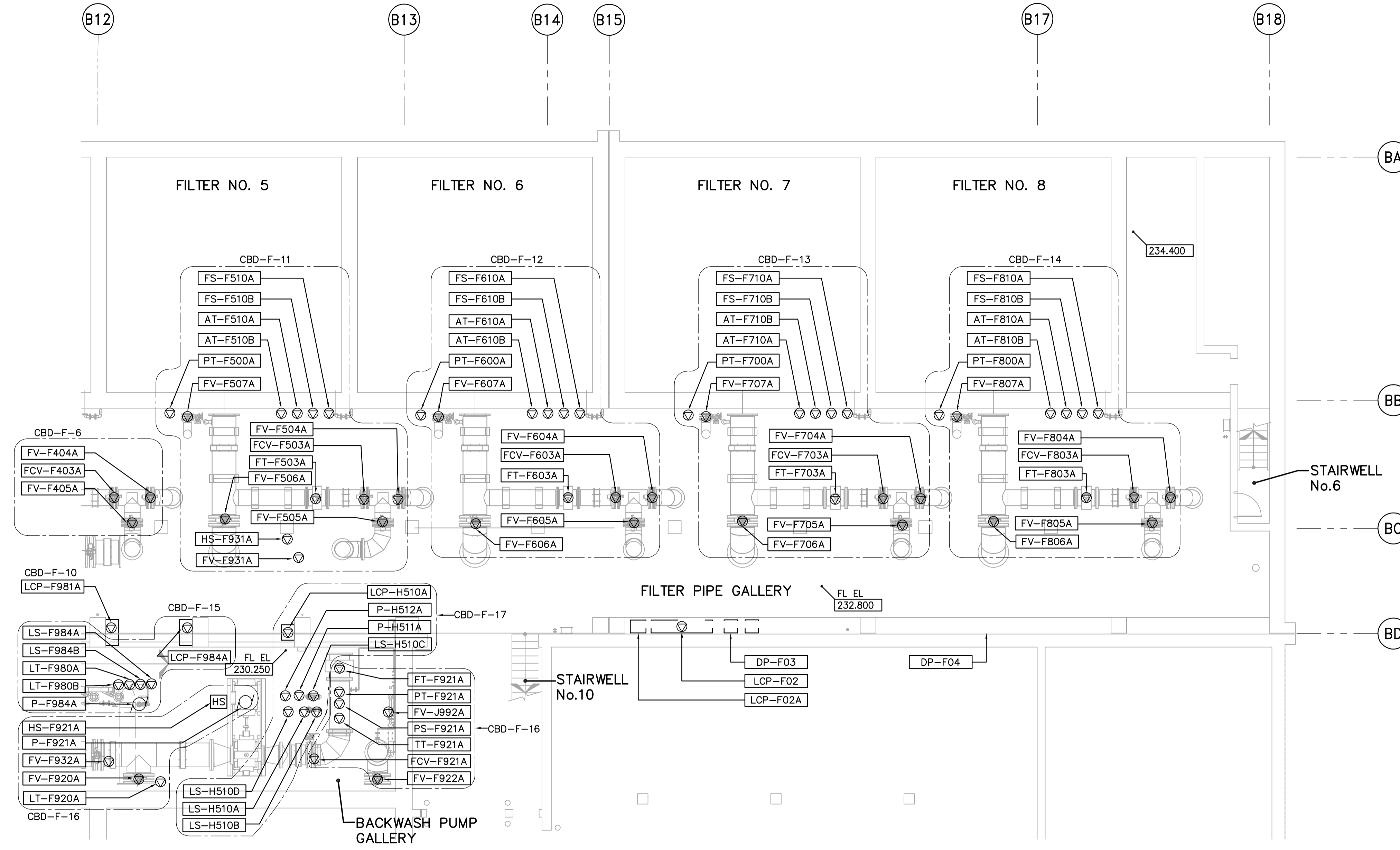
LOWER LEVEL PROCESS PLAN (AREA 2) 1:100
