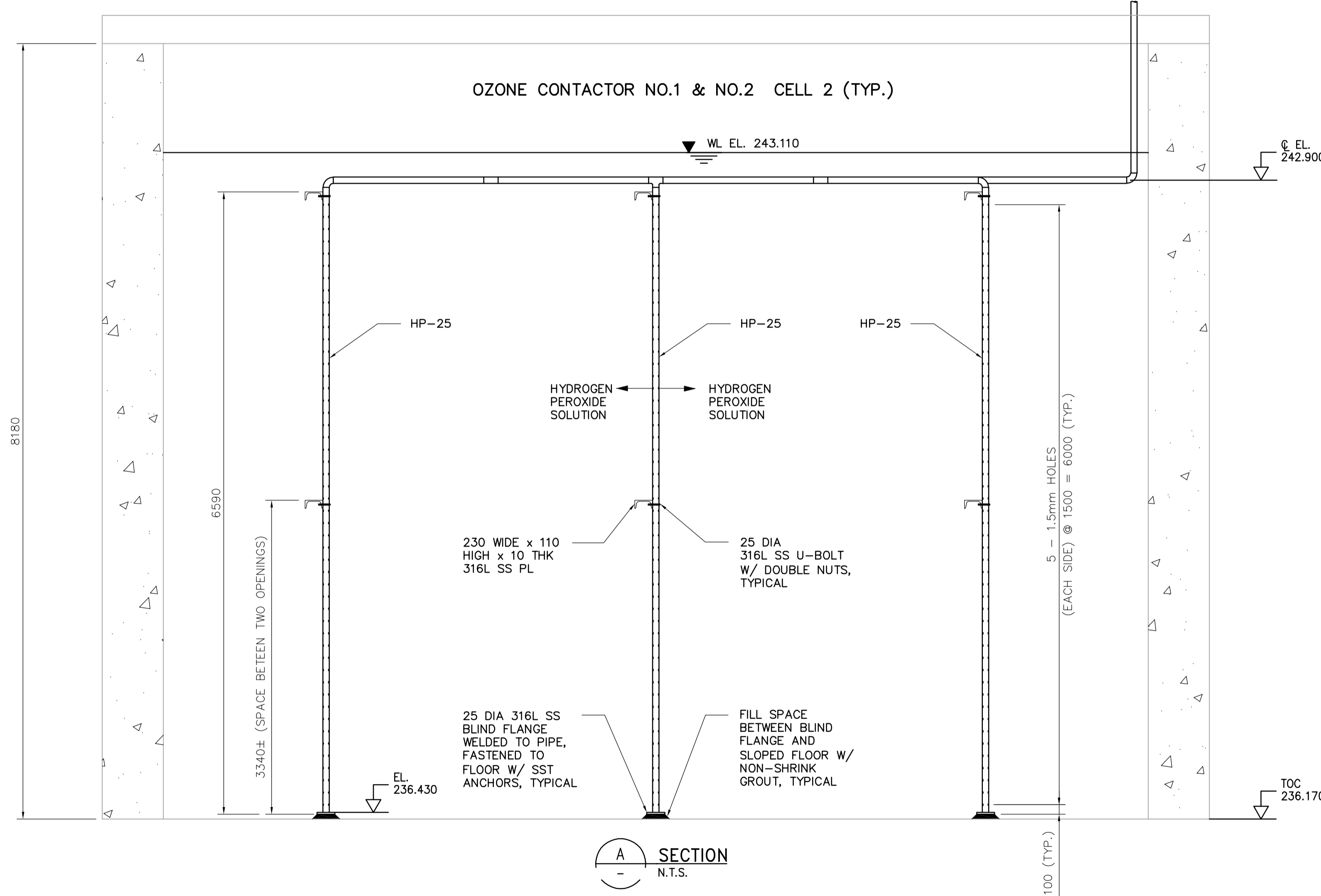
6 OZONE CONTACTOR NO.1 & NO.2 - CELL 2 HYDROGEN PEROXIDE DIFFUSER (TYP.) N.T.S. WO-M0121 WO-M0201 WO-M0203
