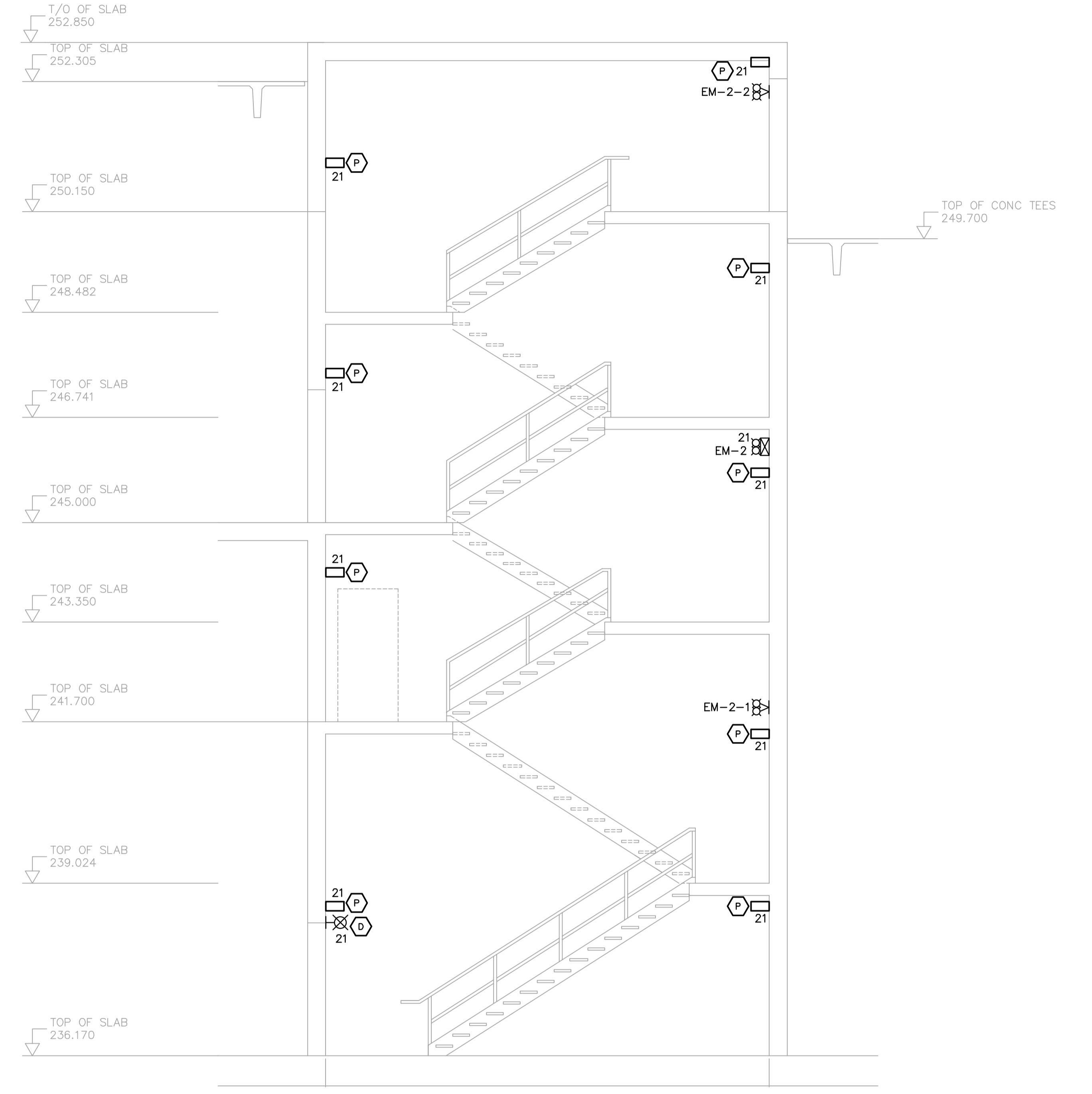
B STAIRWELL NO.8 LIGHTING WC-E0113 1:50 WC-E0123 WC-E0133
